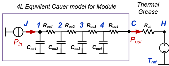
Fig. 5. Equivalent Cauer type thermal network converted from the Foster network shown in Fig.4.
