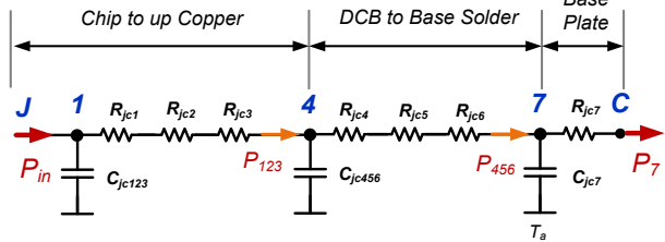
Fig. 8. Transformation of the 7L-Cauer type network to a third order low pass filter according to the frequency behaviours.
