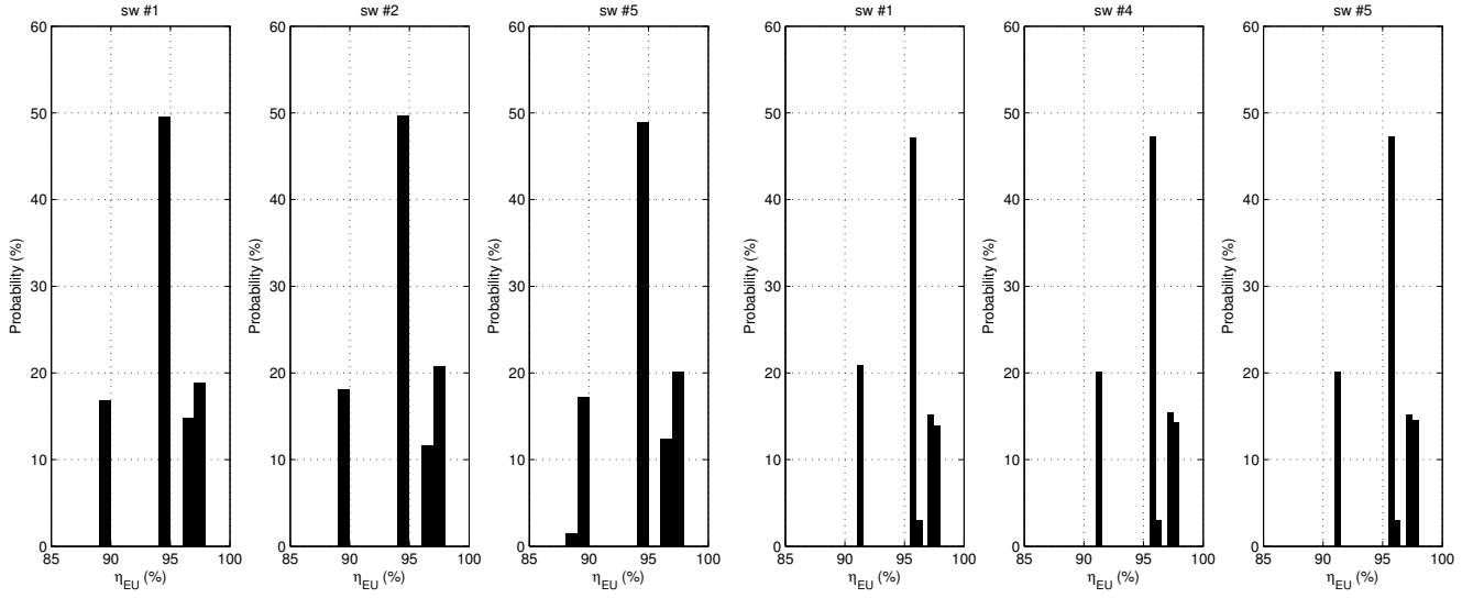
(a) H5. #1: \mu = 94.52\% and \sigma = 2.55\% , #2: \mu = 94.45\% and \sigma = 2.61\% , #5: \mu = 94.41\% and \sigma = 2.66\% . (c) HB-NPC. #1: \mu = 95.33\% and \sigma = 2.23\% , #4: \mu = 95.37\% and \sigma = 2.2\% , #5: \mu = 95.37\% and \sigma = 2.21\% .
