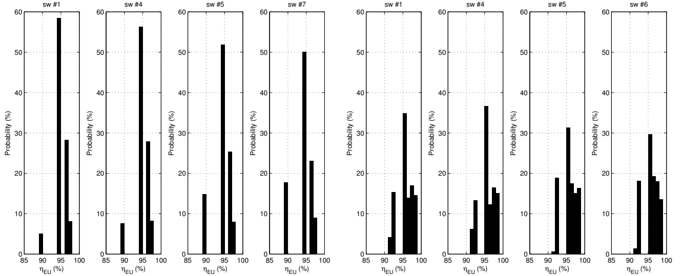
(b) H6. #1: \mu = 95.05\% and \sigma = 1.68\% , #4: \mu = 94.92\% and \sigma = 1.89\% , #5: \mu = 94.51\% and \sigma = 2.33\% , #7: \mu = 94.35\% and \sigma = 2.07\% , #5: \mu = 95.88\% and \sigma = 1.98\% , #6: \mu = 95.86\% and \sigma = 2.48\% . (d) HERIC. #1: \mu = 95.79\% and \sigma = 2.02\% , #4: \mu = 95.76\% and \sigma = 1.97\% .
