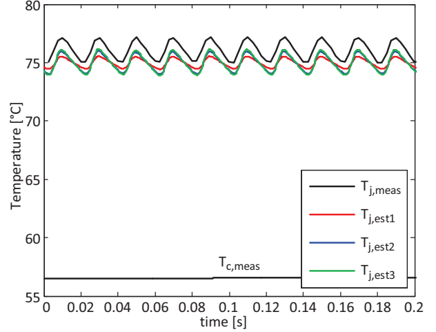
Fig. 13: Measurement: Thermal cycling in the fundamental period (50 Hz) measured and modeled with different number of RC-elements.
