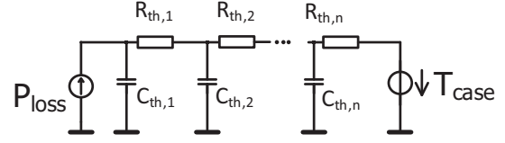
Fig. 3: Cauer network: electric circuit representing the thermal impedance Z_{th,jc} .
