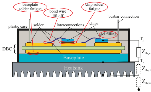
Fig. 1: Scheme of a power electronic module with heatsink, common failures and thermal impedances.
