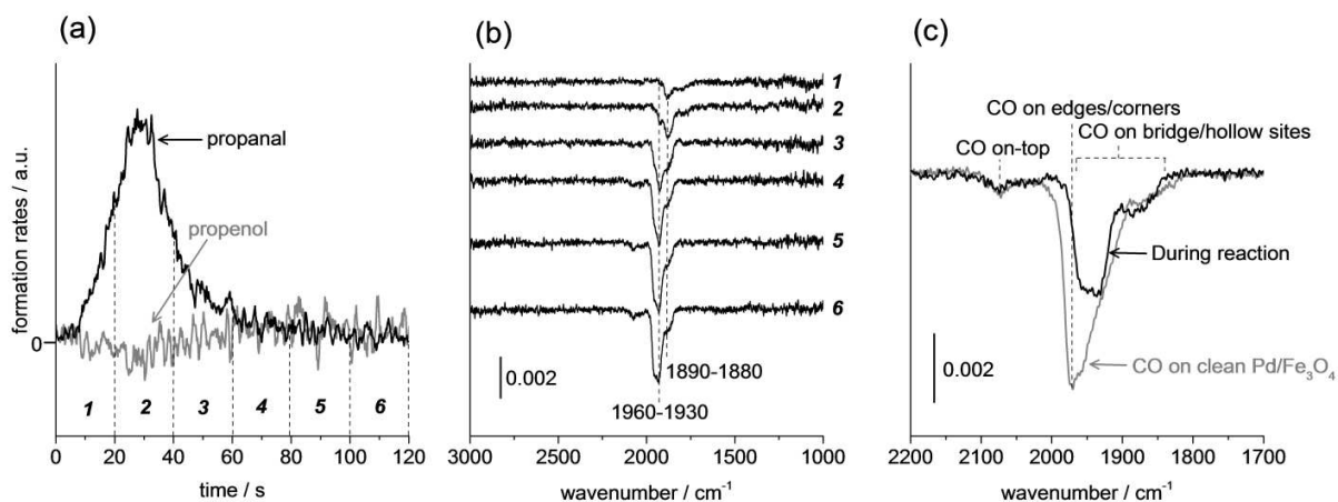
Figure 4. Acrolein hydrogenation over 12 nm Pd/Fe 3 O 4 at 270 K. (a) Gas-phase formation rates of propanal (black) and propenol (grey). (b) Time-resolved IRAS spectra collected during acrolein hydrogenation. Spectra labeled 1-6 were collected during the corresponding regions labeled 1-6 in (a). (c) Comparison of the IRAS spectrum collected during acrolein hydrogenation over 12 nm Pd/Fe 3 O 4 at 270 K (spectrum 6 in (b)) to the IRAS spectrum of CO adsorbed on clean 12 nm Pd/Fe 3 O 4 .
