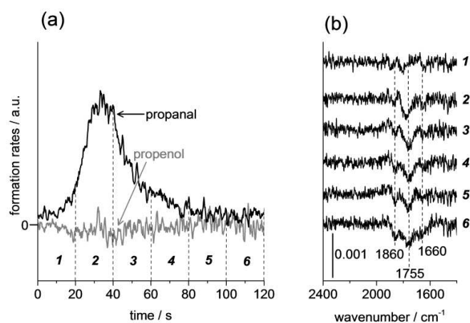
Figure 7. Acrolein hydrogenation over 7 nm Pd/Fe 3 O 4 at 250 K. (a) Gas-phase formation rates of propanal (black) and propenol (grey). Time-resolved IRAS spectra collected during acrolein hydrogenation. Spectra labeled 1-6 were collected during the regions labeled 1-6 in (a).
