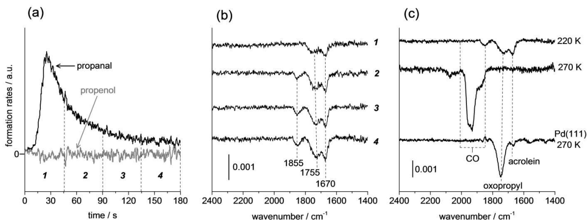
Figure 5. Acrolein hydrogenation over 12 nm Pd/Fe 3 O 4 at 220 K (a) Gas-phase formation rates of propanal (black) and propenol (grey). (b) Time-resolved IRAS spectra collected during acrolein hydrogenation. Spectra labeled 1-4 were collected during the regions labeled 1-4 in (a). (c) Comparison of IRAS spectra collected during acrolein hydrogenation over 12 nm Pd/Fe 3 O 4 at 220 K and 270 K, and over Pd(111) at 270 K.
