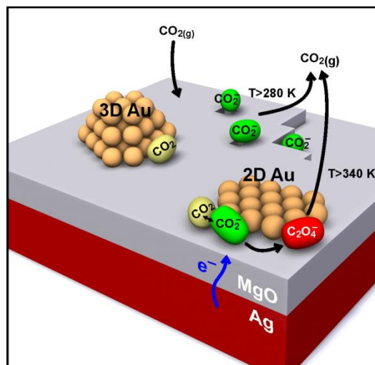
Figure 3: Schematic showing the individual steps of oxalate formation upon chemisorption of \text{CO}_2 on the rim of 2D Au islands on thin \text{MgO}(001)/\text{Ag}(001) films. 22 Carboxylate species (green) are formed both on defect sites of the \text{MgO} film and on the rim of the 2D Au islands by electron transfer. Only on the latter, additional \text{CO}_2 (yellow) is able to solvate the carboxylate species yielding a (\text{CO}_2)_2^- dimer ion, which, after an additional electron transfer, results in adsorbed oxalate \text{C}_2\text{O}_4^{2-} (red). This reaction does not occur on 3D Au particles.
