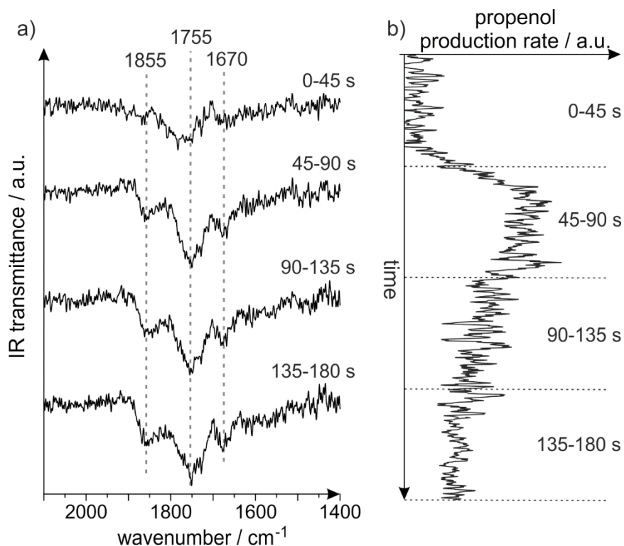
Figure 2: (a) Time-resolved IR spectra monitor the evolution of surface species on 12 nm Pd particles turning over and (b) QMS measurements show the formation rate of propenol in the gas phase simultaneously.
