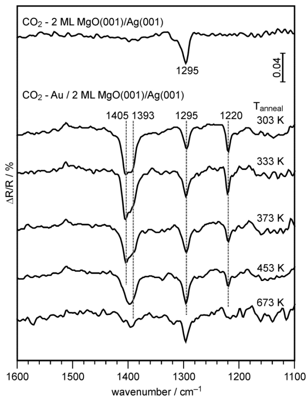
Figure 4: IRA spectra of bare (top) and Au-loaded 2 ML \text{MgO}(001)/\text{Ag}(001) samples recorded after a saturation dose of \text{CO}_2 at 223 K. Au was deposited at 100 K and the samples subsequently annealed to the indicated temperature prior to \text{CO}_2 adsorption.
