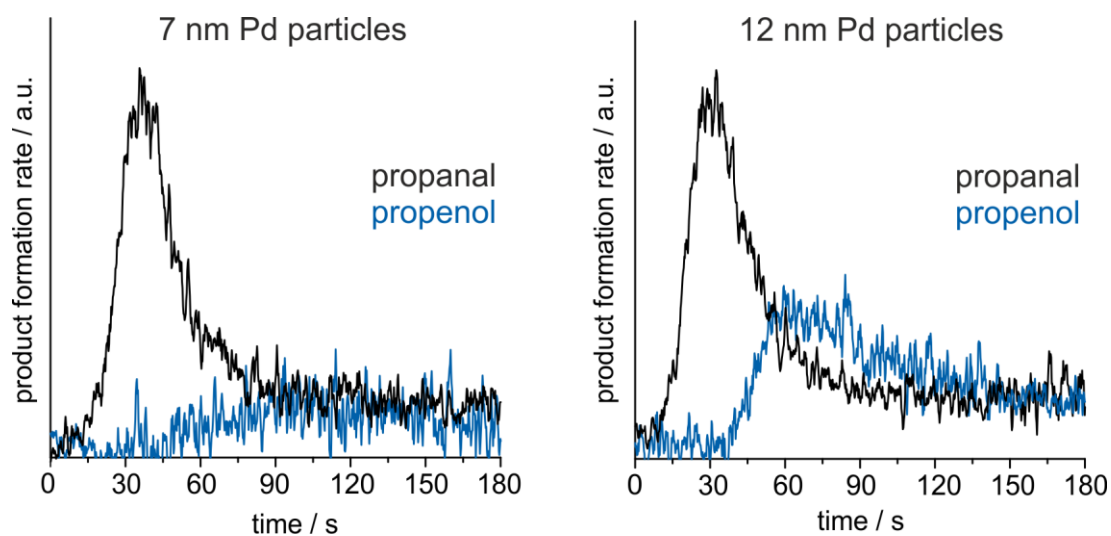
Figure 1: Formation rates of propanal (black lines) and propenol (blue lines) over \text{Fe}_3\text{O}_4 -supported Pd particles with diameters of 7 nm (left) and 12 nm (right) at 250 K detected by QMS.
