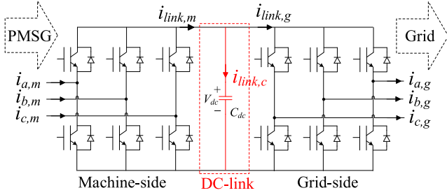
Fig. 1. Two-level back-to-back converter used as a case study.
