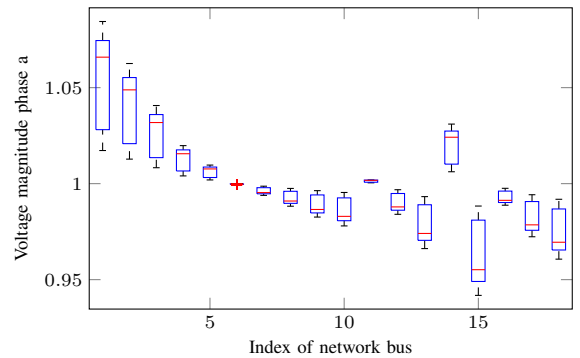
Fig. 8. LV network, Case 1: boxplot of the voltage levels along the buses (phase A) of the LV network in the controlled case.
