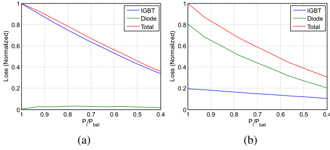
Fig. 5: Loss distribution of the power semiconductor in DABs of the ST (a) Unloaded cell primary side H-bridge (b) Unloaded cell secondary side H-bridge.
