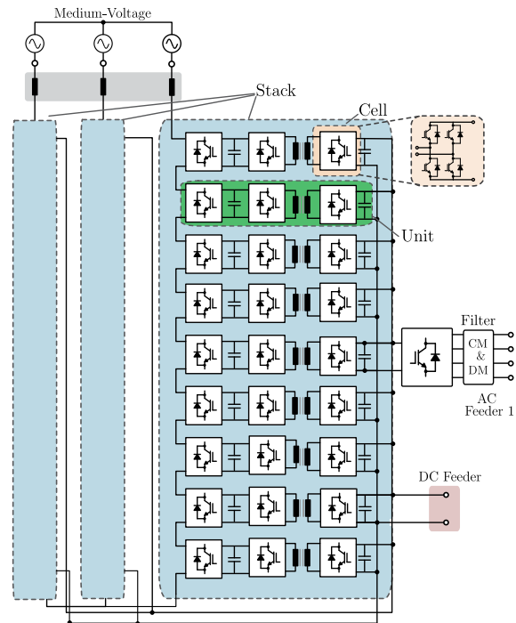
Fig. 1: ST topology with CHB and DAB.
