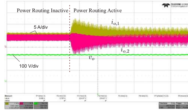
Fig. 13: ST with and without power routing showing the output current of both DAB, ( i_{o,1-2} ) and the output voltage ( v_o ).
