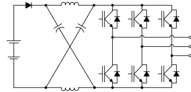
Figure 5. The Z-source inverter [15].
