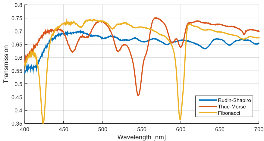
Figure 12: Experimental TE resonance spectra of three nanostructured dielectric waveguides with different deterministic aperiodic nanostructures based on Rudin-Shapiro, Thue-Morse, and Fibonacci binary sequences in water (1.33).
