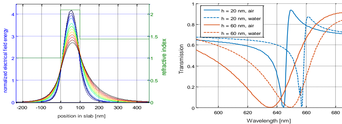
Figure 4: a) Calculated TE 0 mode profiles for wavelengths ranging from 400 nm to 700 nm (color-coded blue to red) of a 100-nm thick high-index layer ( n_2 = 2.2 ) on a quartz substrate. Shorter wavelengths show higher confinement. b) FEM simulation of a 370-nm grating with a 70-nm TiO 2 high-index layer and two different structure depths of 20 nm and 60 nm for two different analytes (air, water).
