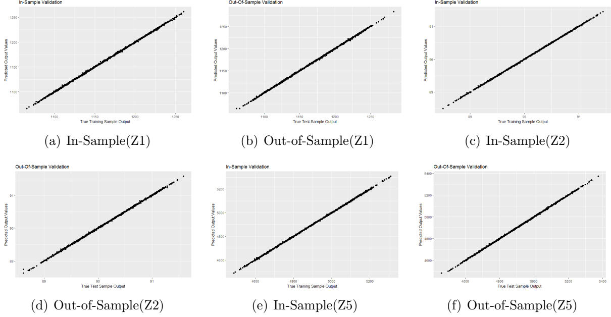
Figure 4: Prediction Performance
