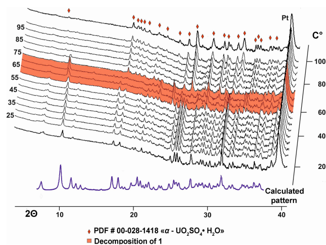
Figure 2. Evolution of the powder diffraction patterns of 1 as a function of temperature. Patterns in the temperature range of decomposition of 1 into “ \text{UO}_2\text{SO}_4 \cdot \text{H}_2\text{O} ” (PDF # 00-028-1418) are marked in red.
