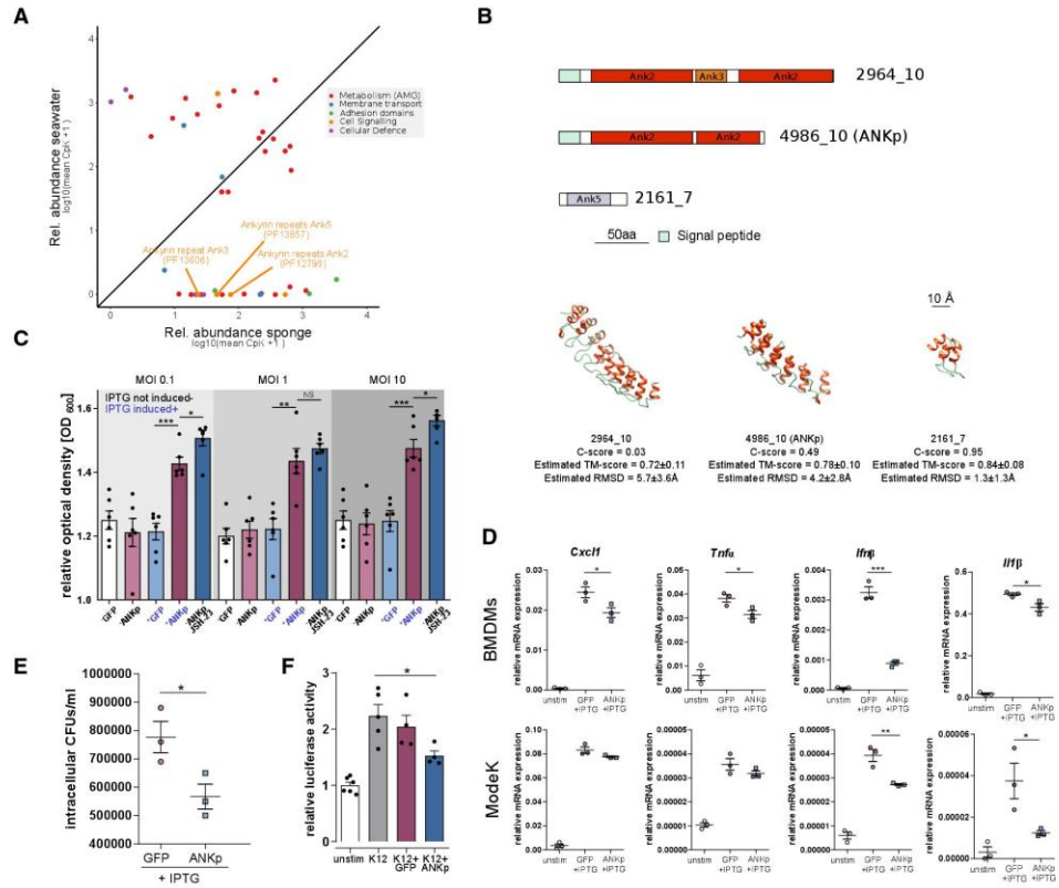
Figure 3. Symbiont Phage ANKp Reduces Phagocytosis and Immune Response of Eukaryote Cells toward Bacteria
