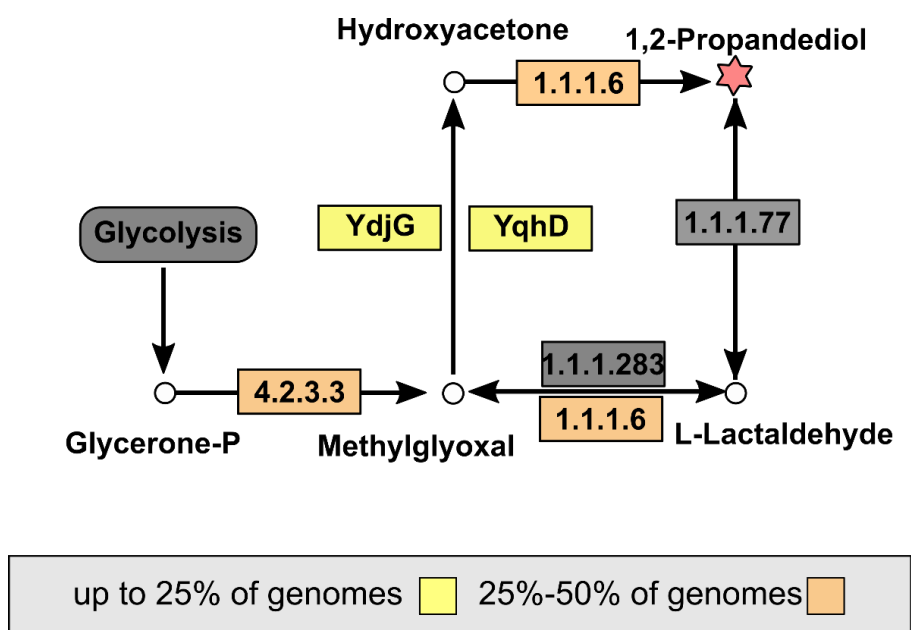
Figure B3-I: Propionate metabolism leading to 1,2 Propanediol. 145 bacterial and archaeal genomes with ecosystem annotation “Porifera” or “sponge” were selected in the IMG database (as of Oct 2019) and their annotated functions were mapped to the propionate metabolism (KEGG:map00640) using the Integrated Microbial Genomes & Microbiomes(IMG/M) system interface (Chen et al., 2019).
