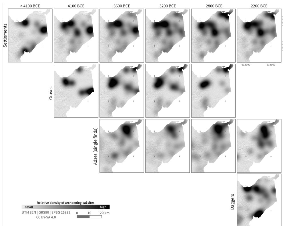
Figure 5. Absolute location differences as reflected by density differences in archaeological sites during Neolithic transformation phases (Rows indicate the different archaeological sources and context; columns correspond to the different Neolithic phases, whose starting dates are shown. The utilized archaeological sample corresponds to all finds that belong to the different phases.).
