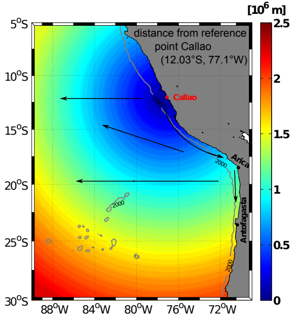
Figure 2.6: Distance from the reference point Callao ( 12.03^{\circ}\text{S} , 77.1^{\circ}\text{W} ) for each point in lat.-lon.-space in the ETSP. The arrows denote simplified tracer transport directions to give their context to the Hovmoeller diagrams in Figs. 2.7 & 3.6-3.9.
