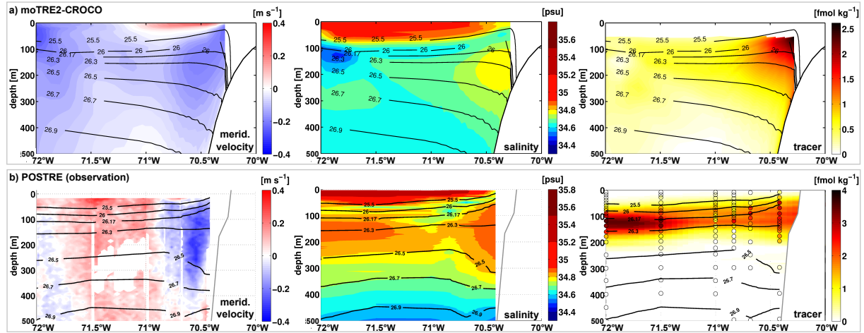
Figure 3.12: Aligning the tracer to the PCUC exemplary along 21^{\circ}\text{S} 17 months after injection for (a) moTRE2-CROCO, and (b) POSTRE; via meridional velocity, salinity and tracer concentration. Please note the different color axis for the tracer concentration.
