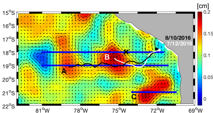
Figure 3.13: Eddies measured during the tracer survey with SLA (shaded) on 17. March 2017 with ship position (x) during survey cruise. Two eddies (A, B) tracked backward (white and black track) to their origin (dot). Sections of observed tracer and hydrography shown in Fig. 3.14 indicated. (Schütte, F., 2017 - personal correspondence)
