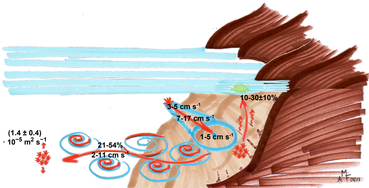
Figure 6.1: Summarizing the relevant processes governing the tracer distribution and their quantified effect on the tracer in the ETSP. The tracer and its behavior is indicated in red; shelf/land in brown, the water (including its motions: PCUC, and eddies) in blue.
