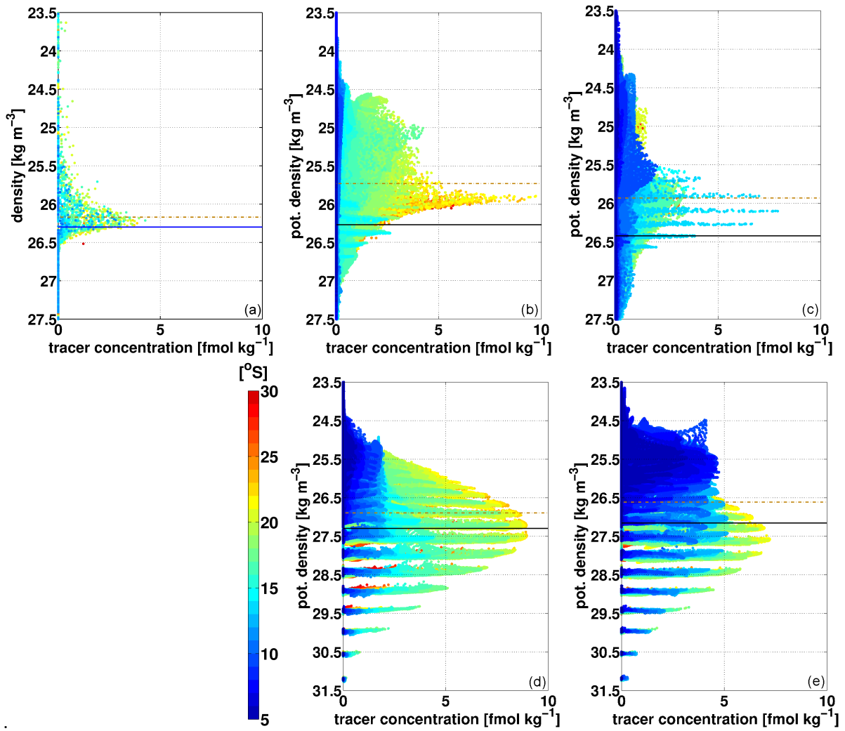
Figure A.2: Tracer density distribution for (a) POSTRE, (b) moTRE1-ROMS, (c) moTRE2-CROCO, (d) moTRE3-NEMO, (e) moTRE4-NEMO. Injection depth indicated as blue/black line, the tracer weighted mean dash dotted in brown. Note the different y-axis for NEMO.
