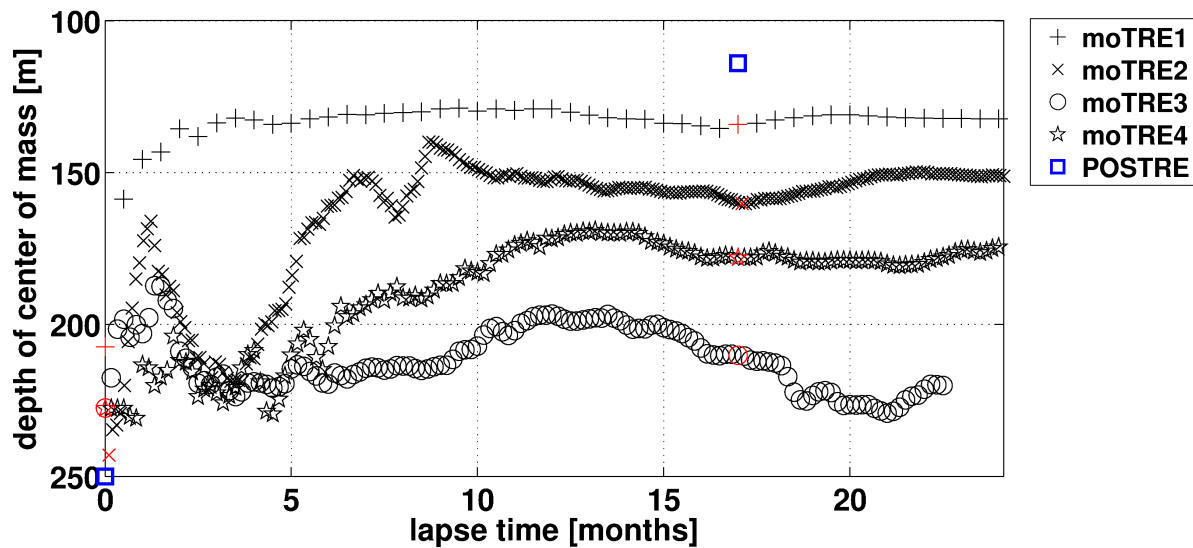
Figure 4.9: Tracer weighted mean depth over time.
