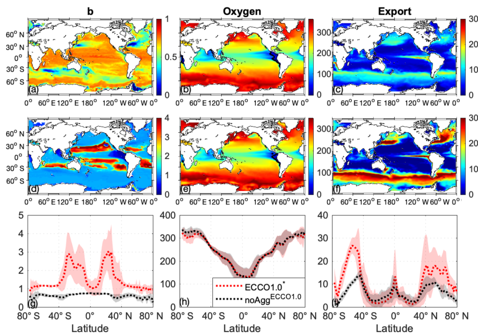
Figure 1. Global maps of b (a, d), O_2 at 100 m ( \text{mmol m}^{-2} , b, e) and export at 100 m ( \text{mmol P m}^{-2} \text{ a}^{-1} , c, f) for \text{noAgg}^{\text{ECCO1.0}} (a, b, c) and for the best aggregation model with regard to the sum of J_{\text{RMSE}} and J_{\text{OMZ}} (simulation no. 26; d, e, f). The black line indicates the OMZ for a criterion of 50 \text{ mmol m}^{-3} . Lower panels: Global mean (dotted line) and standard deviation (transparent shaded) of b (g), O_2 (h) and export (i) of \text{noAgg}^{\text{ECCO1.0}} (black) and the best aggregation model with regard to the sum of J_{\text{RMSE}} and J_{\text{OMZ}} (simulation no. 26; red). Please note the different scaling for b values (a, d).
