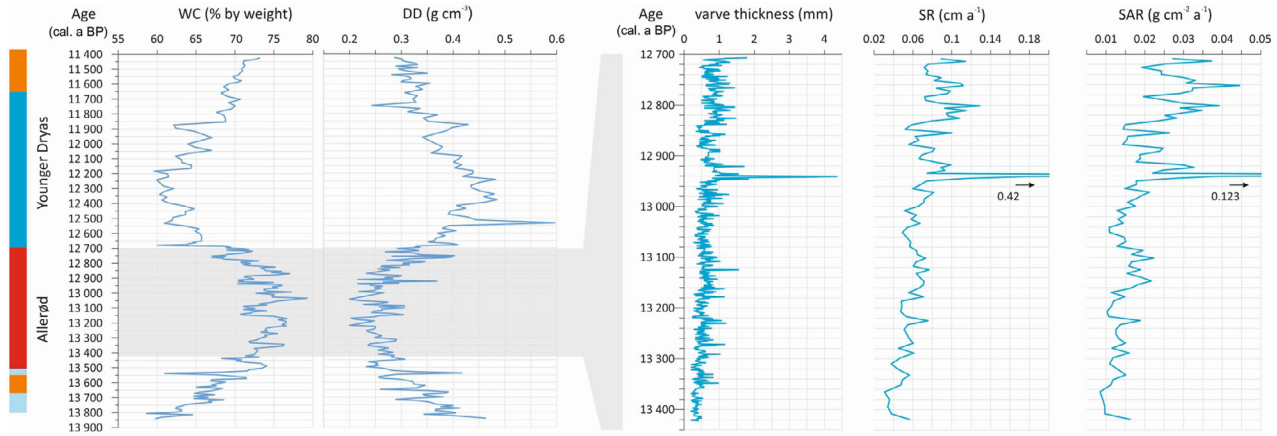
Fig. 4. Allerød and Younger Dryas section of the Nahe palaeolake sediment sequence. Left: water content (WC) and dry density (DD); right: varve thickness, sedimentation rate (SR) and sediment accumulation rate (SAR).
