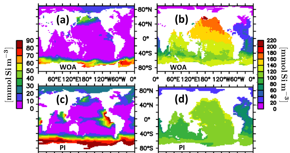
Figure A1. Surface and deep (2,000 m to bottom average) DSi concentrations in units of mmol Si/m 3 . Panels (a) and (b) refer to surface and abyssal observations (Garcia, Locarnini, Boyer, & Antonov, 2010), respectively. Panels (c) and (d) refer to simulated preindustrial ( PI ) surface and abyssal concentrations, respectively.
