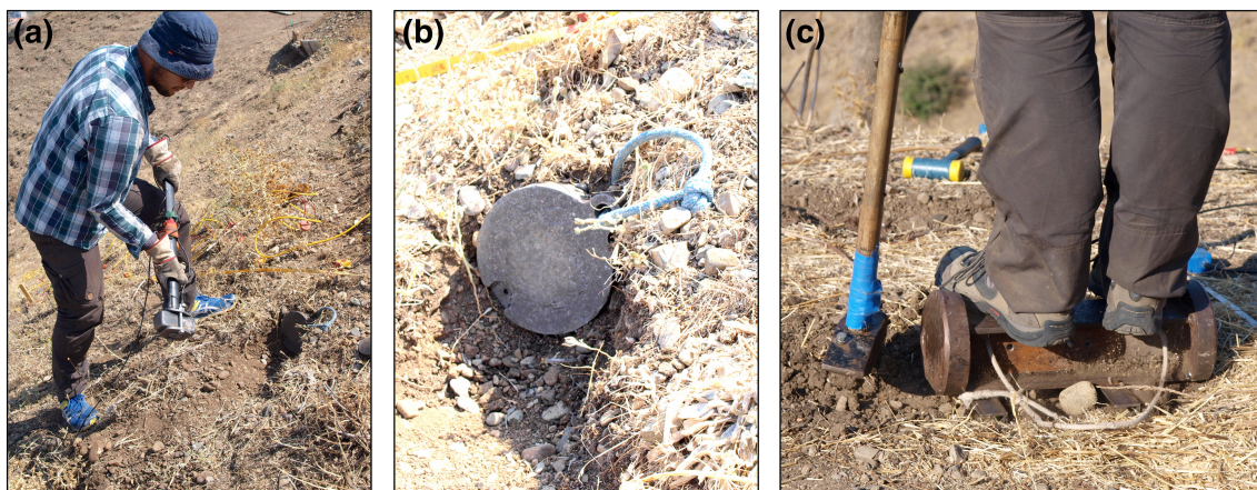
FIGURE 4 SH-sources: (a) Hammer blow on a vertically standing (a, b) iron plate or an (c) iron bar (photography by W. Rabbel, September 2015 [b, c] and September 2017 [a]) [Colour figure can be viewed at wileyonlinelibrary.com ]
