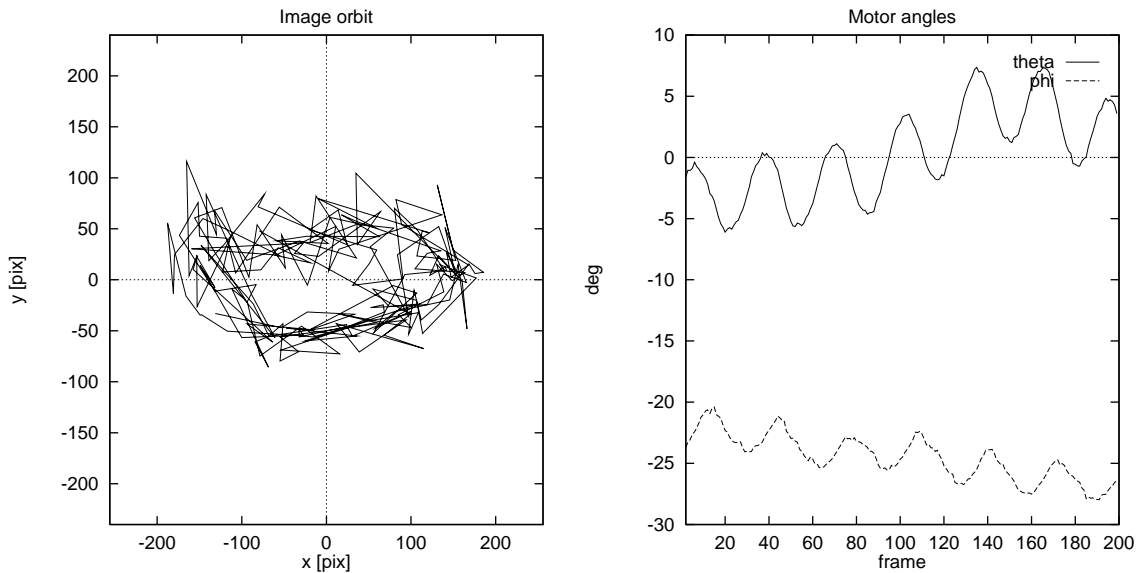
Figure 12. The camera is pursuing a target mounted on the gripper of a manipulator while the camera is itself translating forwards. The target is moving on a circle with frequency 0.70 Hz. The translation of the camera is shown in the shift of the angle oscillation center. As the camera is approaching on the left side of the manipulator it must turn more to the right (positive shift in vergence) and more downwards (negative shift in tilt).
