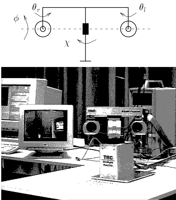
Figure 1. The four degrees of freedom of the camera platform (top) and how it looks like (bottom).
