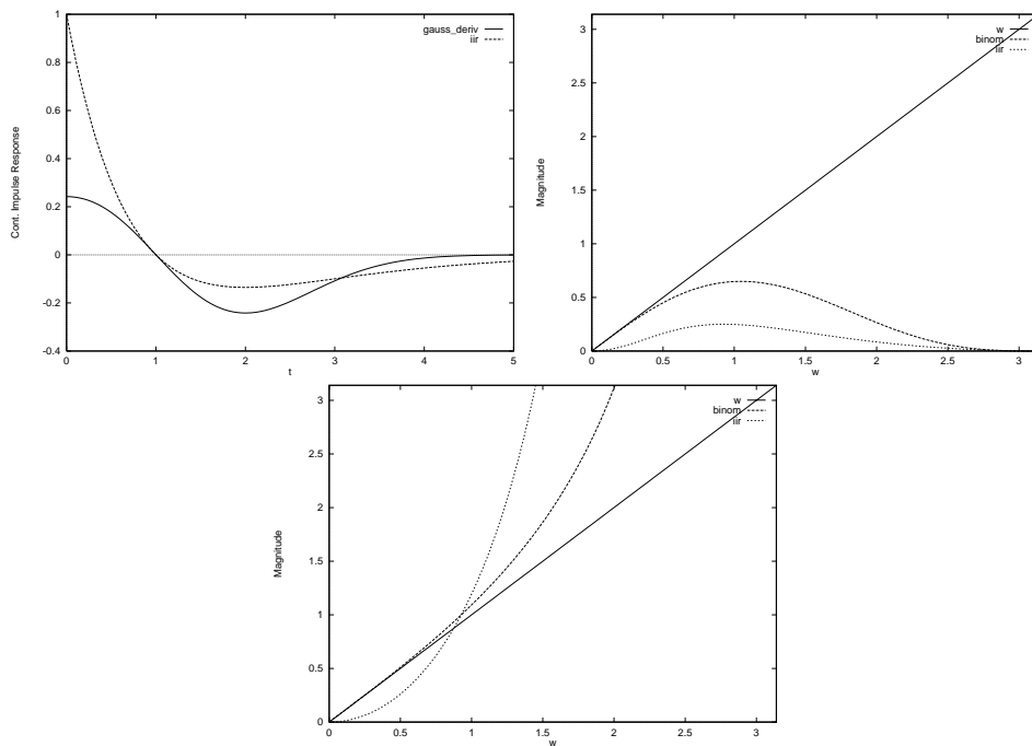
Figure 3. Continuous impulse response comparison of the shifted first derivative of a Gaussian ( \sigma = 1 ) and the IIR second order derivative filter ( \tau = 1 ) (above). In the middle we show the frequency responses of the 5-points binomial approximation of the first Gaussian derivative and the IIR second order derivative filter ( \tau = 1 ). Below we show the pure differentiation effects, i.e. the same spectra divided by the frequency responses of the low-pass prefilters.
