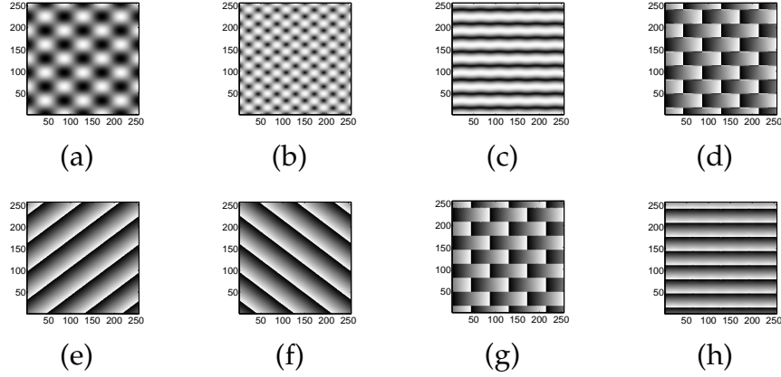
Figure 3: Example 1: 2-D input signal f with \omega_1 = 6\pi, \omega_2 = 8\pi (a). Local amplitude according to f_{tot} (b). Local amplitude (c) and phase (d) wrt. f_{part}^1 . Local phase wrt. f_{so1} (e) and f_{so2} (f). \phi (g) and \theta (h) resulting from f_{so}^q .
