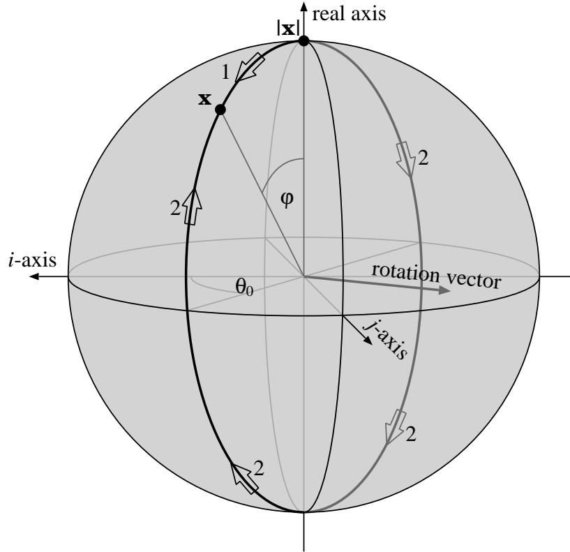
Figure 6: Phase representation using a rotation vector \varphi . First the real value |\mathbf{x}| is rotated about the second axis ( j -axis) by \varphi , and second about the third axis (real axis) by \theta_0 . The rotation vector is orthogonal to the plane spanned by the real axis and the vector \mathbf{x} . Its length is given by the angle between the real axis and \mathbf{x} . Although the rotation vector is unique, the decomposition is not. There are two possibilities: 1. (\theta_0, \varphi) and 2. (\theta_0 + \pi, -\varphi) .
