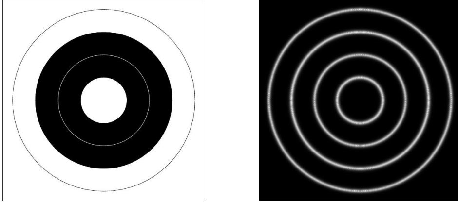
Figure 3: Left: test image showing all even and odd symmetries for all orientations; right: the energy of the corresponding monogenic signal is isotropic and independent of the local symmetry.
