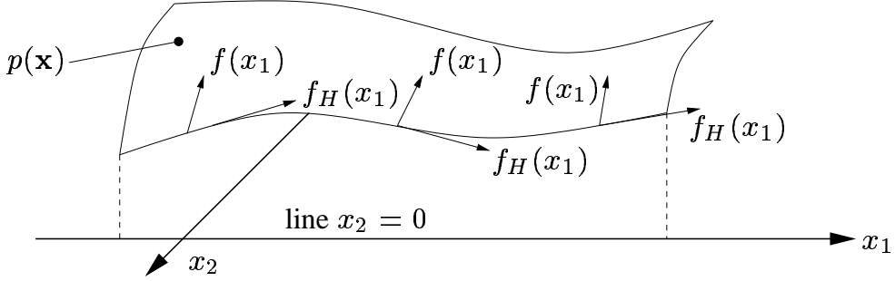
Figure 1: Harmonic potential p(\mathbf{x}) for x_2 < 0 and its gradient field on the boundary x_2 = 0 , which is given by the 1D function f(x_1) and its Hilbert transform f_H(x_1) .
