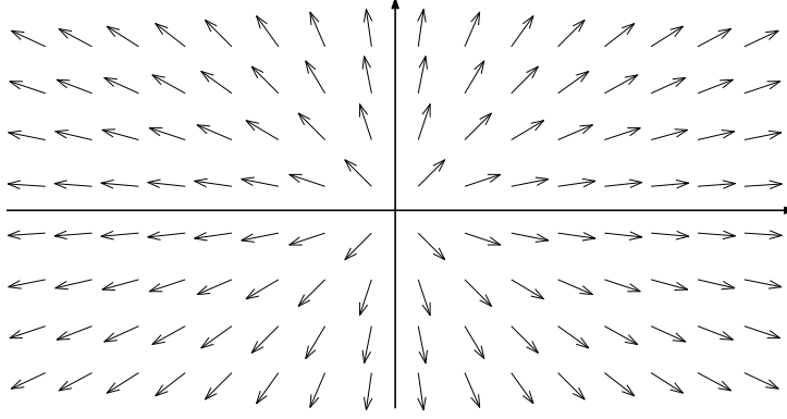
Figure 2: Transfer function of the Riesz transform displayed as a vector field. The axes are the frequencies u_1 and u_2 . The vector field is given by the normalized frequency vectors (see (10)) and by setting it to zero at the origin (see text).
