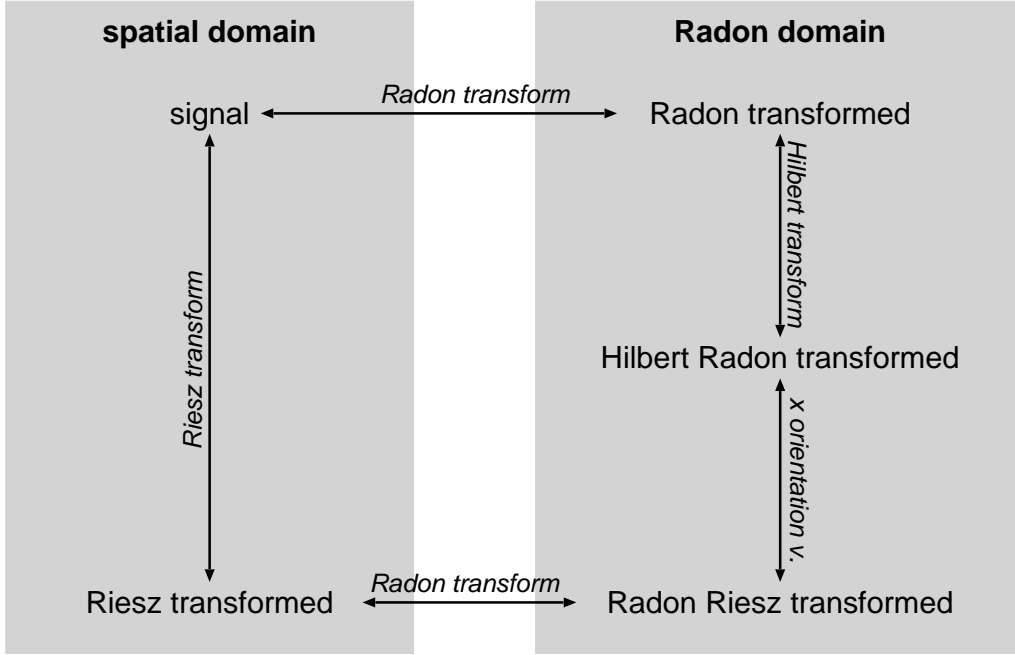
Figure 5: The relation between Radon, Riesz, and Hilbert transform. The Riesz transform in the spatial domain (left) is equivalent to the Hilbert transform with subsequent multiplication by the orientation vector in the Radon domain (right).
