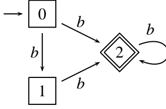
Figure 1: alternating Büchi automaton
