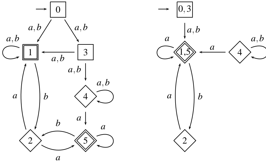
Figure 5: automaton and de-semi-elective quotient
