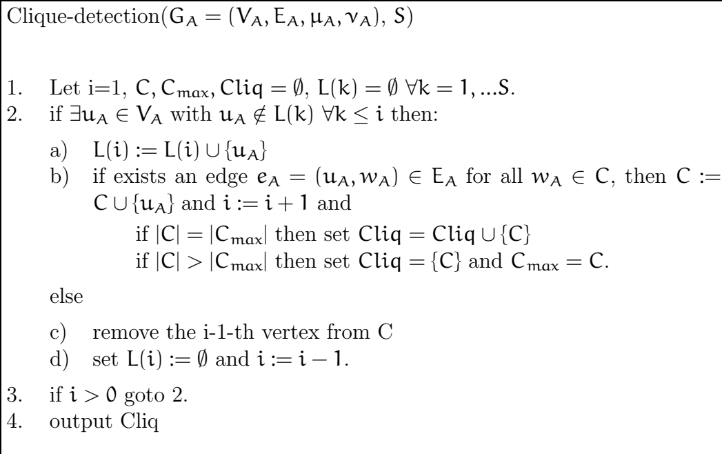
Figure A.2: Algorithm for clique detection.
