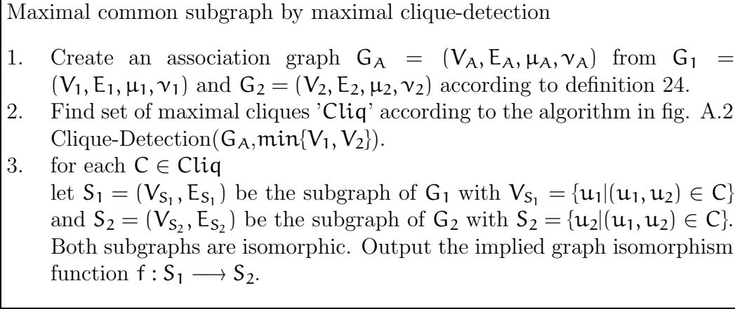
Figure A.1: Graph-matching based on clique detection.
