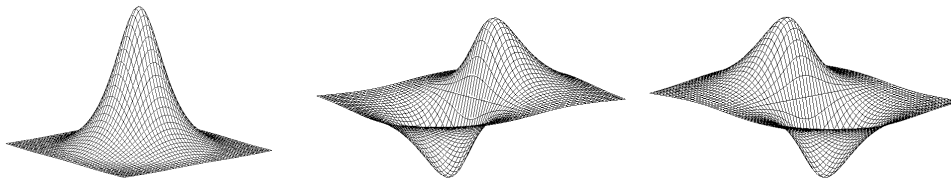
Fig. 2.2: From left to right: the Poisson kernel ( h_P ) and the two components of the conjugate Poisson kernel ( h_{Q1} and h_{Q2} ). Note that the two components of the conjugate Poisson kernel constitute one single isotropic operator.
