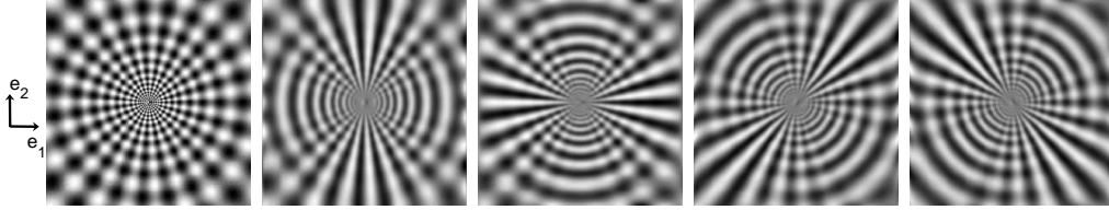
Fig. 3.2: From left to right are the test image, 1D signals result from the angular windowing functions of \cos^2(\alpha) , \cos^2(\alpha - \frac{\pi}{4}) , \sin^2(\alpha) and \sin^2(\alpha - \frac{\pi}{4}) , respectively.
