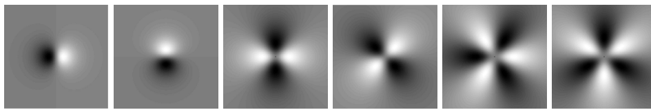
Fig. 2.1: From left to right are spherical harmonic bandpasses of order 1 to 3 in the spatial domain, every spherical harmonic consists of two orthogonal components. White indicates positive one and black represents negative one.
