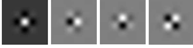
Fig. 5.2: Four components of the quaternionic Gabor filter.
