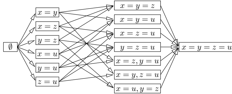
Figure 2: Variable identification graph with four variables
