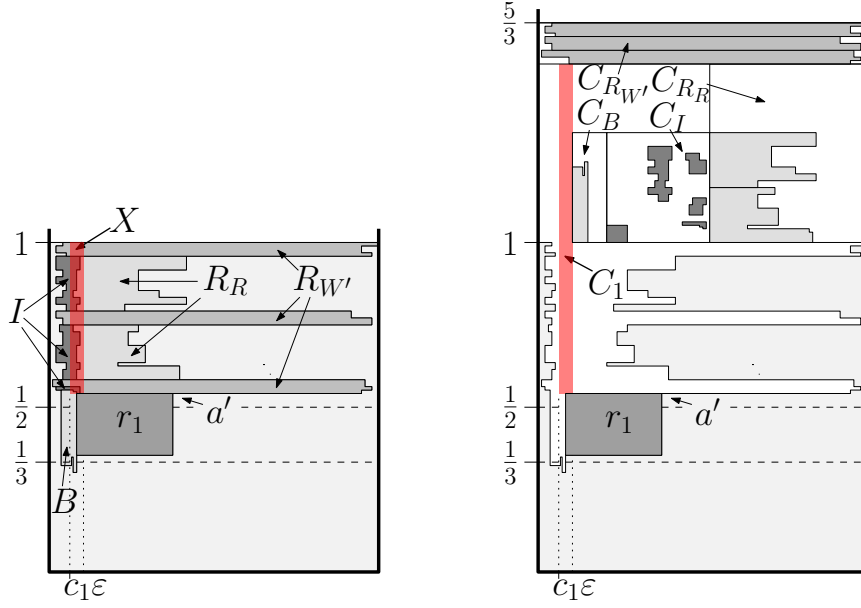
(a) Definition of R_{W'} , R_R , B and I (here in Case 1 with a' + h' \leq 1/6 ) (b) Modified packing where C_1 is packed in the red slot of height 1 and width \varepsilon .
