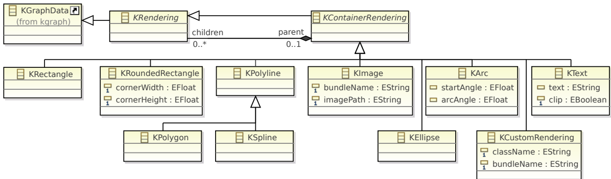
Figure 3.6: KRendering primitives to be composed to diagram figures.
