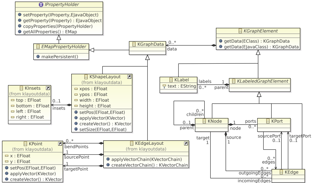
Figure 3.5: KGraph meta model with basic graph structures and layout data.
