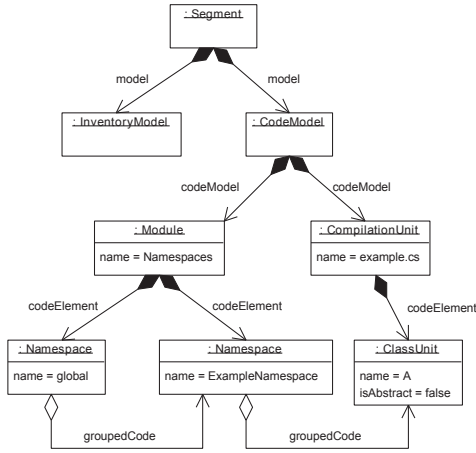
Figure 4: Simplified, visualized KDM instance generated from Listing 2 in the phase P1
