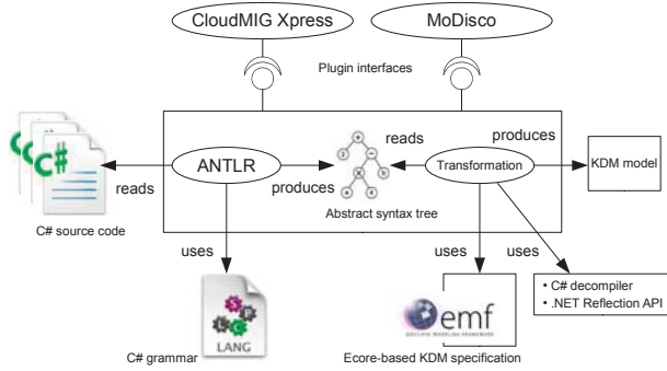
Figure 2: Transformation architecture
