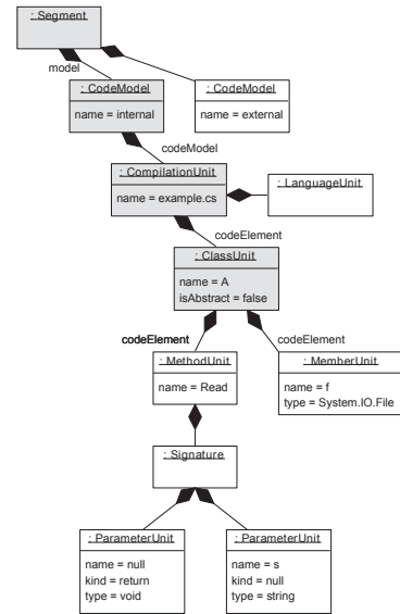
Figure 5: Simplified, visualized KDM instance generated from Listing 2 in the phases P1 and P2. Elements created in P1 are colored gray, elements from P2 are colored white.
