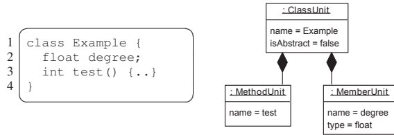
Figure 1: A C# example and a corresponding, simplified KDM instance
