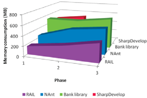
Figure 7: Memory consumption of the four applications within the three phases
