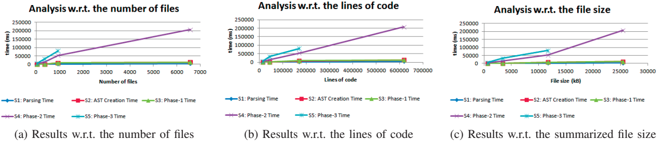
Figure 8: Analysis results w.r.t. the three different project size metrics
