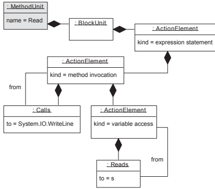
Figure 6: Simplified, visualized KDM instance generated from Listing 2 in the phases P1 to P3
