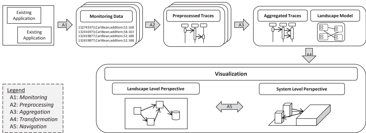
Figure 1: ExplorViz approach taken from [FWWH13]
