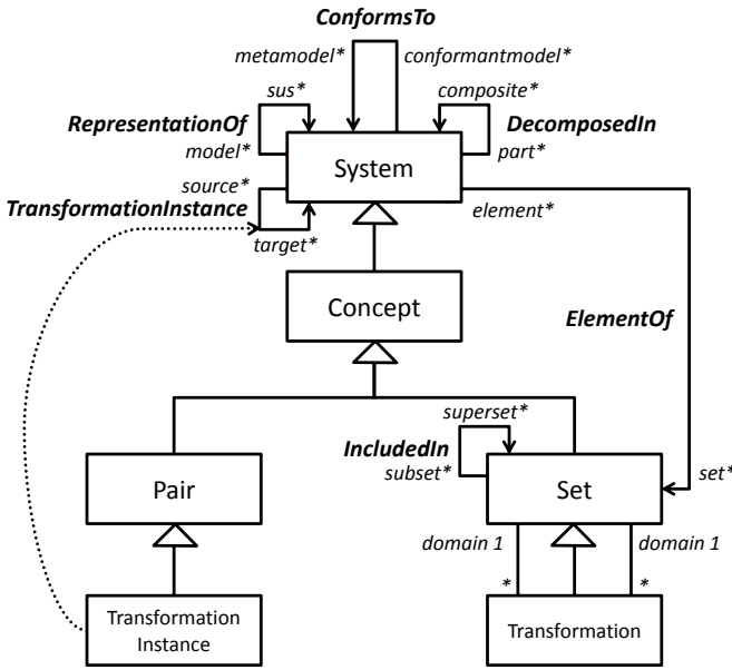
Figure 4.2. The MDSO metamodel (megamodel metamodel) based on Favre and NGuyen [2005].
