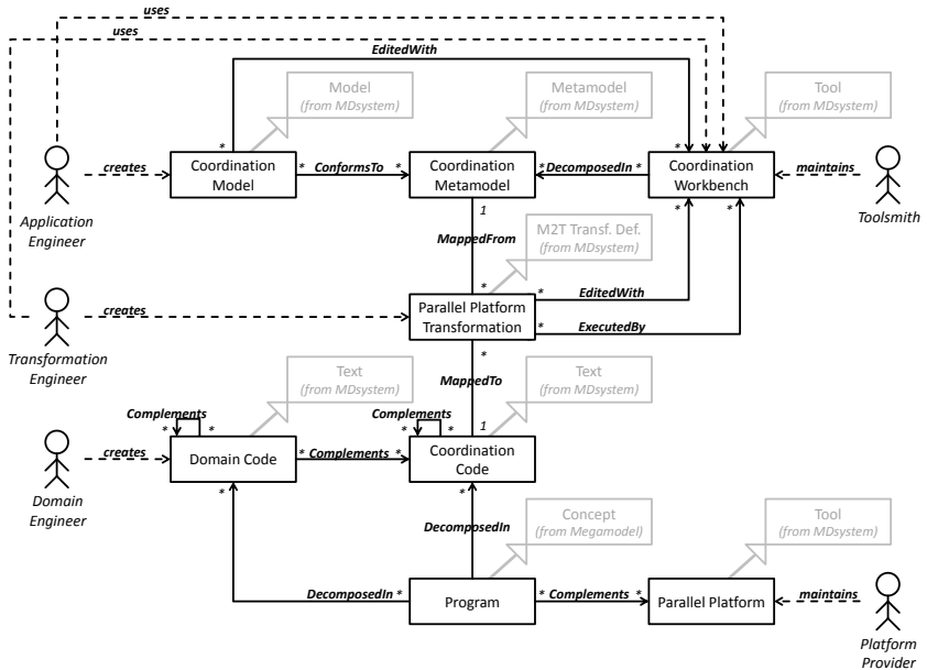
Figure 5.1. The Coordination Engineering metamodel as a specialisation of the MD system metamodel from Section 4.3.
