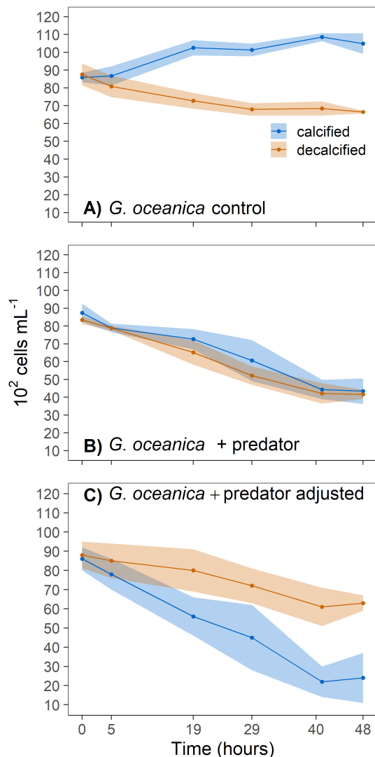
Figure 3 | Mean concentrations \pm 1SD (ribbons) of calcified and decalcified G. oceanica within the mixed treatment. Decalcified cells produced new coccoliths in the dark and the re-calcified cells were progressively enumerated as calcified cells (compare Fig. 2). This is why the concentrations of calcified cells increased in the controls (A). B) shows the decrease of the cell concentrations in the presence of A. tonsa and C) displays the values of B corrected with the controls (see main text for detail).
