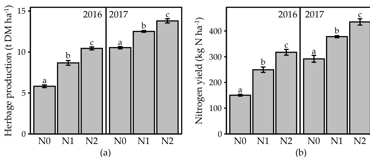
Figure 1. (a) Annual herbage dry matter production and (b) nitrogen yield in 2016 and 2017 for three N application rates (0 (N0), 140 (N1) and 280 (N2) \text{kg N ha}^{-1} ). Mean values with different superscripts differ between N application rates ( p \leq 0.05 ).
