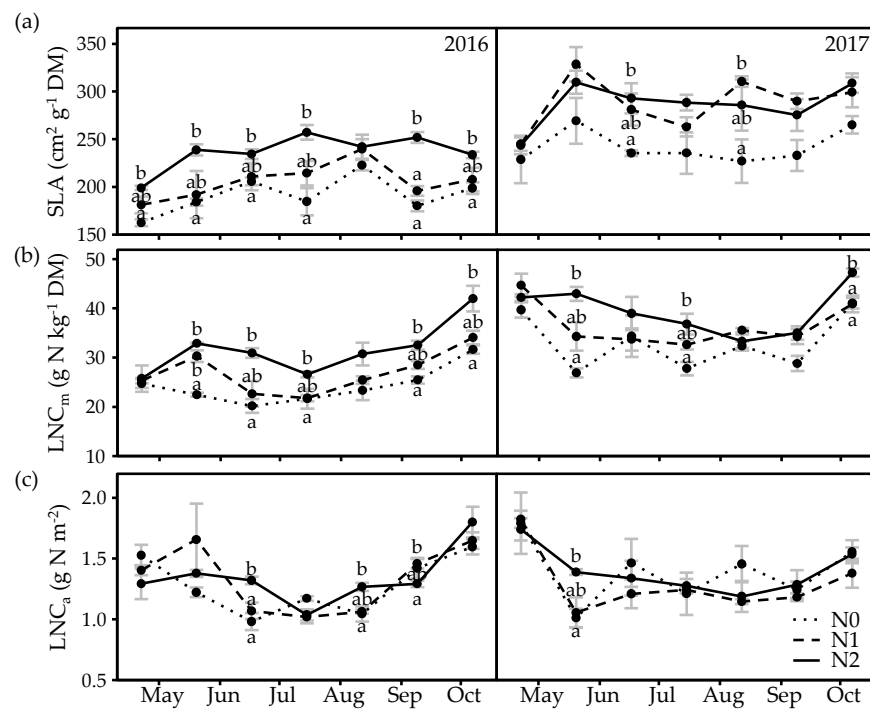
Figure 5. (a) Specific leaf area (SLA), (b) leaf nitrogen content per unit mass (LNC m ) and (c) leaf nitrogen content per unit area (LNC a ) during the vegetation period of 2016 and 2017 for three N application rates (0 (N0), 140 (N1) and 280 (N2) kg N ha -1 ). Mean values at the same date with different superscripts differ between N application rates ( p \leq 0.05 ). Error bars show the standard error of the mean for the interaction between defoliation date and N application rate.
