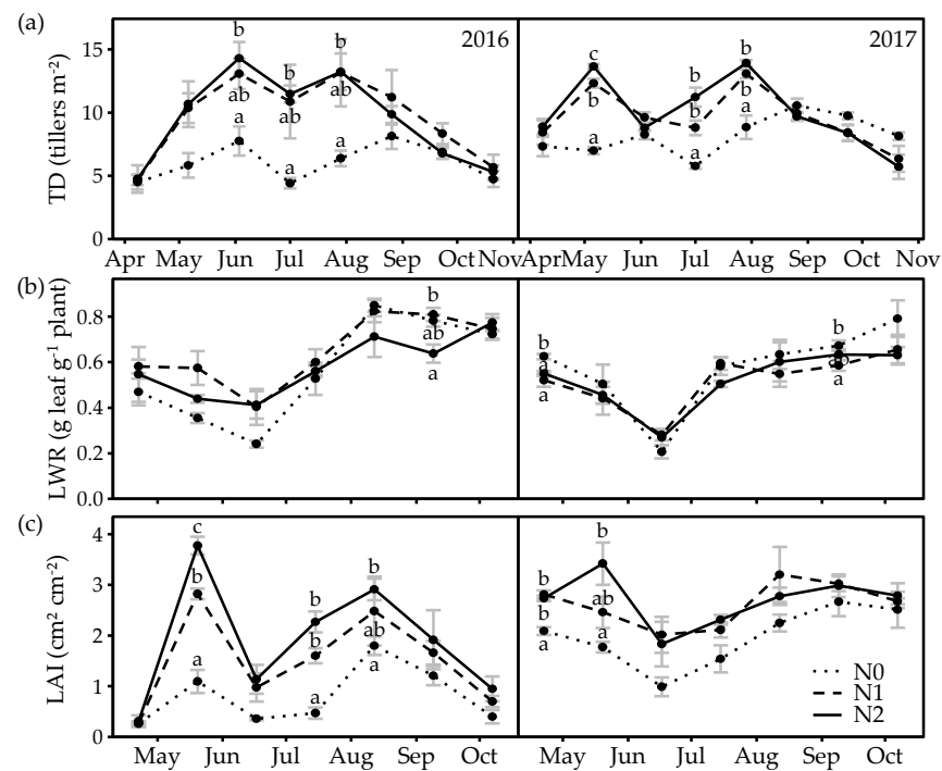
Figure 4. (a) Tiller density (TD), (b) leaf weight ratio (LWR) and (c) leaf area index (LAI) during the vegetation period of 2016 and 2017 for three N application rates (0 (N0), 140 (N1) and 280 (N2) kg N ha -1 ). Mean values at the same date with different superscripts differ between N application rates ( p \leq 0.05 ). Error bars show the standard error of the mean of the interaction between defoliation date and N application rate.
