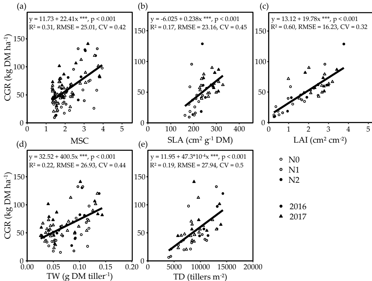
Figure 6. Linear relationships between crop growth rate (CGR) and (a) mean stage by count (MSC), (b) specific leaf area (SLA), (c) leaf area index (LAI), (d) tiller weight (TW) and (e) tiller density (TD) for three N application rates (0 (N0), 140 (N1) and 280 (N2) kg N ha -1 ) across two years (2016 and 2017).
