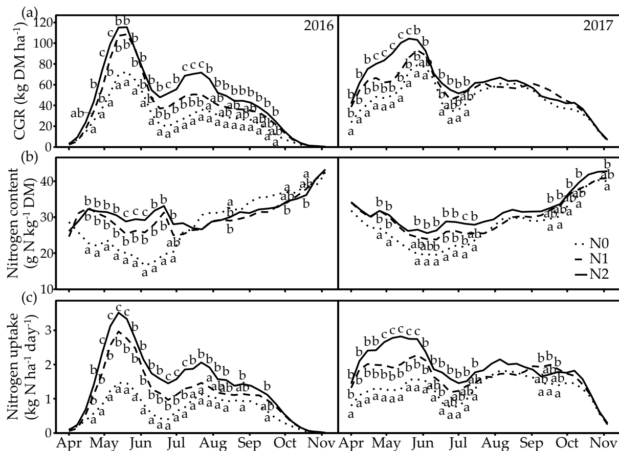
Figure 2. (a) Mean daily crop growth rate (CGR), (b) mean nitrogen content and (c) mean daily nitrogen uptake of the total herbage harvested during the vegetation period of 2016 and 2017 for three N application rates (0 (N0), 140 (N1) and 280 (N2) kg N ha -1 ). Mean values at the same harvest date with different superscripts differ between N application rates ( p \leq 0.05 ).
