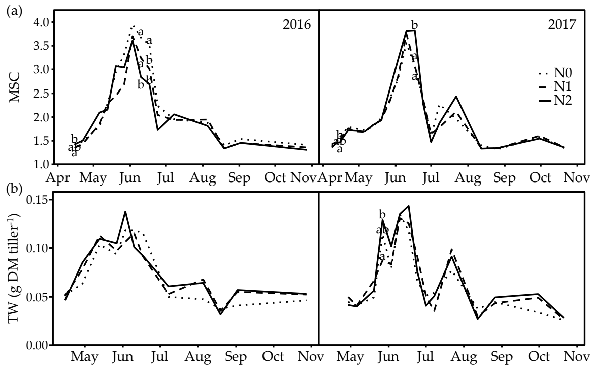
Figure 3. (a) Mean stage by count (MSC) and (b) tiller weight (TW) during the vegetation periods of 2016 and 2017 for three N application rates (0 (N0), 140 (N1) and 280 (N2) kg N ha -1 ). Mean values at the same date with different superscripts differ between N application rates ( p \leq 0.05 ).
