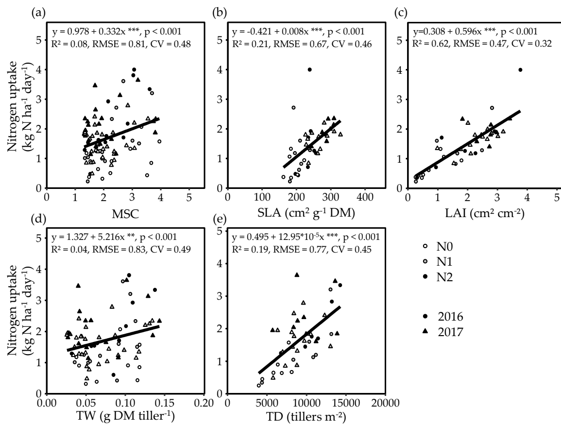
Figure 7. Linear relationships between daily nitrogen uptake and (a) mean stage by count (MSC), (b) specific leaf area (SLA), (c) leaf area index (LAI), (d) tiller weight (TW) and (e) tiller density (TD) for three N application rates (0 (N0), 140 (N1) and 280 (N2) kg N ha -1 ) across two years (2016 and 2017).
