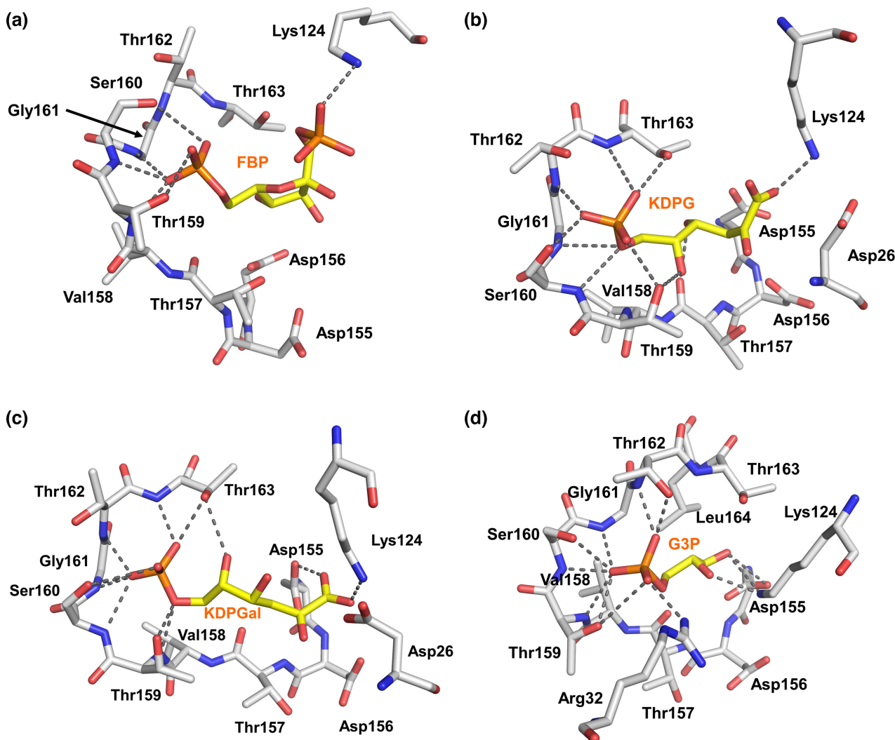
FIGURE 8 Molecular docking of effector molecules into the homology model of Haloferax volcanii GfcR. Only the region of GfcR corresponding to the PRPP-binding site of OMP synthase is shown where the effector molecules are predicted to bind. The panels are as follows: (a) Fructose-1,6-bisphosphate (FBP), (b) 2-keto-3-deoxy-6-phosphogluconate (KDPG), (c) 2-keto-3-deoxy-6-phosphogalactonate (KDPGal) and (d) Glycerol-3-phosphate (G3P). Potential hydrogen or electrostatic bonds are shown as dashed lines. Effector molecules are colored in yellow bonds and the GfcR residues in the binding site are gray.
