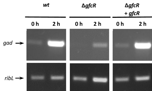
FIGURE 4 GfcR dependent transcription of gad encoding gluconate dehydratase of Haloferax volcanii analyzed by RT-PCR. Cells of wild-type, \Delta gfcR mutant and the mutant complemented with gfcR in trans ( \Delta gfcR + gfcR ) were pre-grown on 0.2% casamino acids and expression of gad was induced by 5 mM D-glucose. Formation of gad transcripts was monitored before (0h) and 2h after the addition of D-glucose (2h). The ribL gene encoding the ribosomal protein L10 was used as constitutive expression control.
