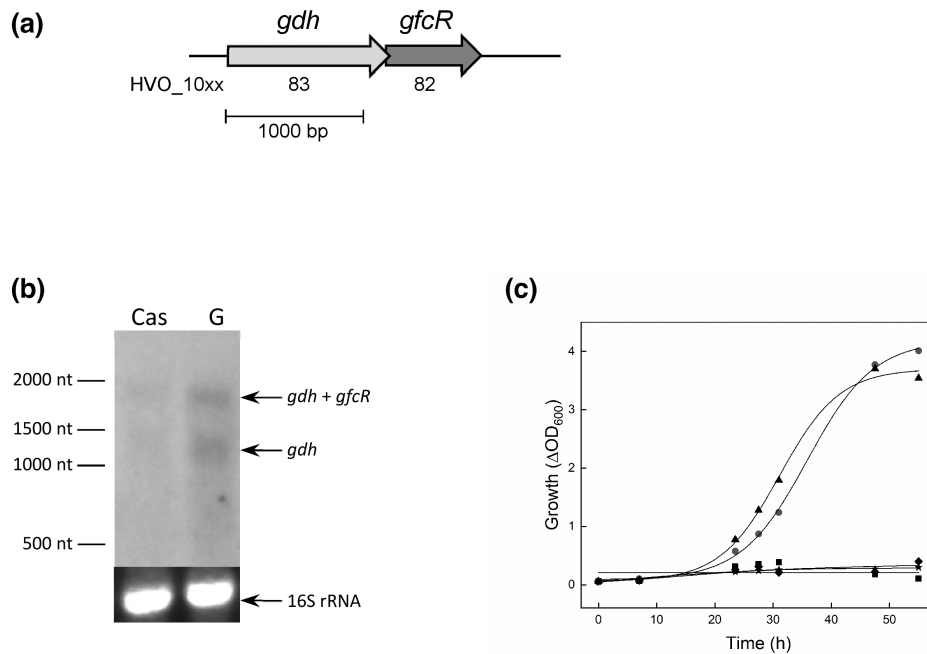
FIGURE 2 Transcriptional analysis of the gdh-gfcR operon and growth of the Haloferax volcanii \Delta gfcR mutant on D-glucose. (a) Genomic view of the gdh-gfcR operon. (b) Northern blot analysis with RNA from cells grown on casamino acids (Cas) or D-glucose (G) using a probe against gdh (HVO_1083). 16S rRNA was used as loading control. (c) Growth on 25 mM D-glucose of the \Delta gfcR mutant (square), wild-type (circle) and the deletion mutant that was complemented with gfcR (triangle), gfcR - \Delta\alpha 1 (diamond) or gfcR - \Delta\alpha 1\alpha 2 (asterisk).
