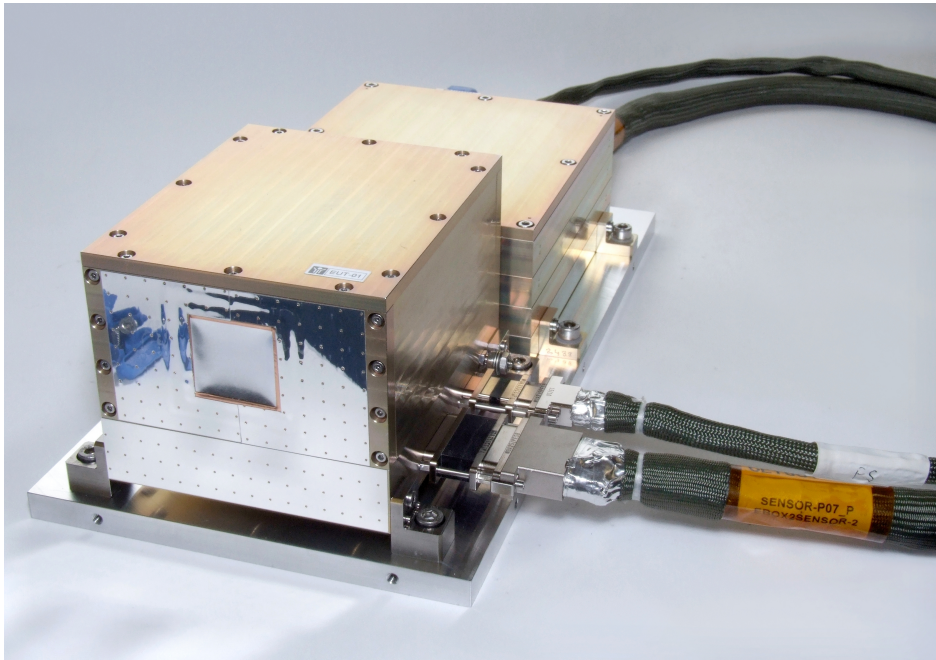
Figure 10: A photograph of the LND, including the sensor head (SH) in the front, electronic box (EB) in the rear, and 1-meters data and power harness that connects the SH and EB. The figure was adapted from Wimmer-Schweingruber et al. (2020) and shows the flight spare model of LND and was taken on 2018.11.23.
