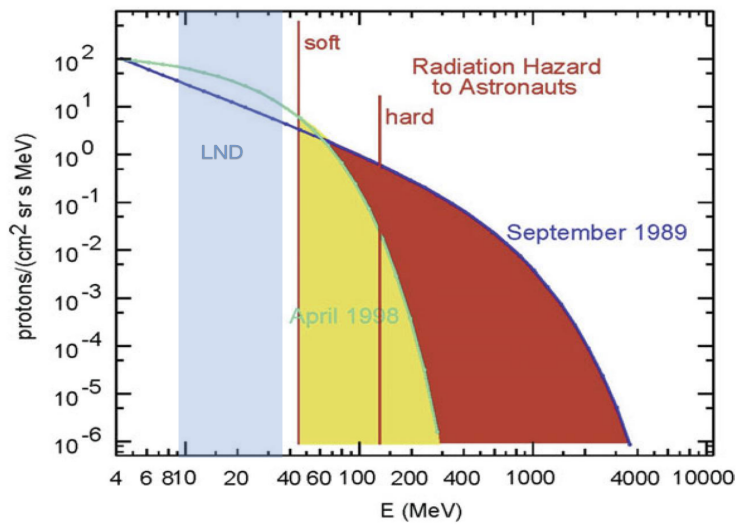
Figure 9: The proton spectra of two famous SEP events. The yellow and red colored regions indicate the energy region with protons harmful to instruments and the human body. Both "hard" and "soft" spectra threaten human activities. The blue-colored region indicates the energy coverage of LND stopping particles in the energy range of 8 - 35 MeV. (Figure reproduced and adapted from Reames (2021))
