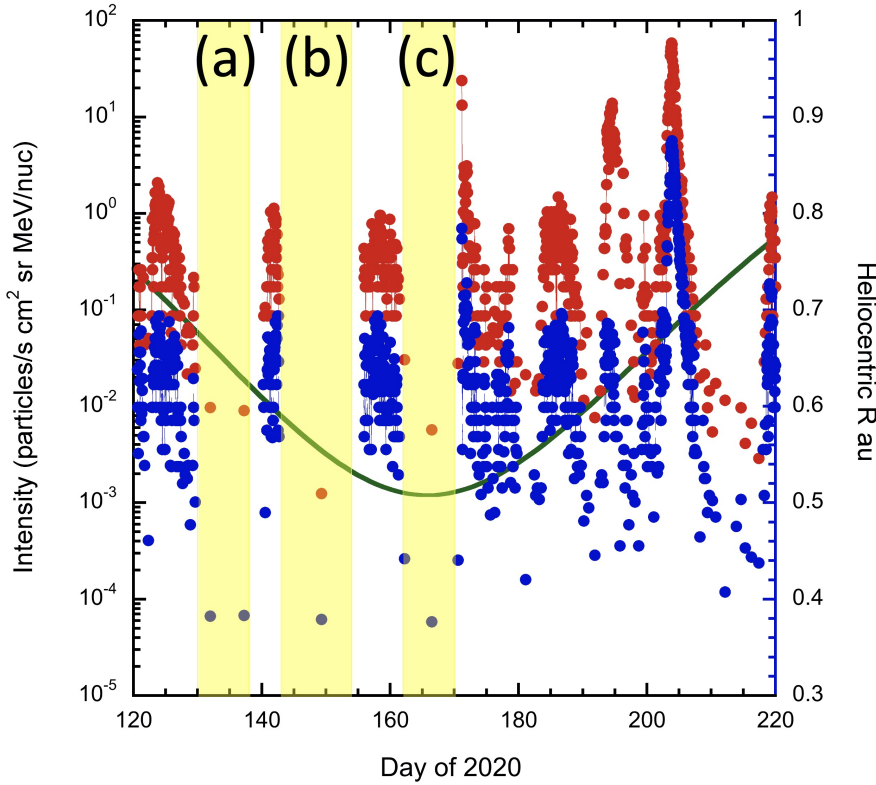
Fig. B.1. Intensities of 273 keV nucleon ^{-1} H (red filled circles) and He (blue), for mid-2020 showing heliocentric distance and yellow intervals (a)–(c) with low intensities. Large intensity increases in the figure are associated with CIRs and SEP events. The text describes residual time variations in intervals (b) and (c) that led them to be disqualified, leaving interval (a) as the super-quiet interval.
