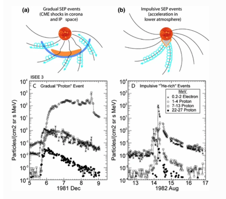
Figure 2: Two classes of SEP events. (a) The gradual SEP events that are associated with CME driven shocks in the corona or in the interplanetary space. The particles populate the interplanetary magnetic field (IMF) lines over a wide range of longitudes. (b) The impulsive SEP events that are associated with solar flares. Here, the particles only populate a limited range of the open IMF lines that are well-connected to the flare site. Plots (c) and (d) are the corresponding typical proton and electron time profiles of the large gradual and small impulsive SEP events. The figure is reproduced from Desai and Giacalone (2016).
