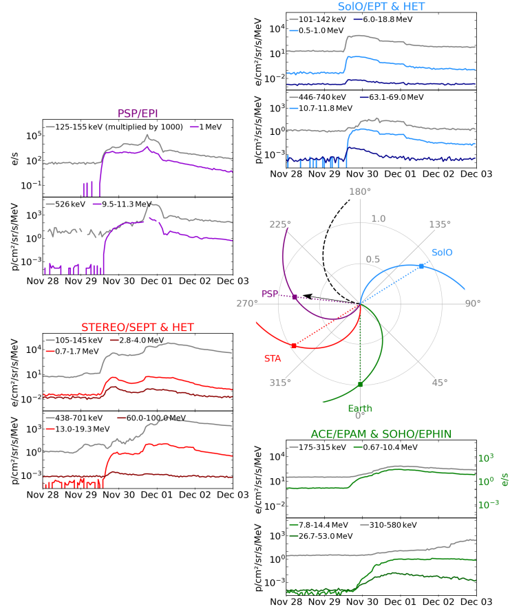
Figure 3: The first wide-spread solar energetic particle event on Nov 29, 2020. The central panel illustrates the locations of different spacecraft and their magnetic connections to the Sun. Both proton and electron observations from Solar Orbiter (SolO) (top), Parker Solar Probe (PSP) (top left), Solar Terrestrial Relations Observatory (STEREO)-A (bottom left), and the Earth including Advanced Composition Explorer (ACE) and Solar and Heliospheric Observatory (SOHO) are given. (Figure reproduced from Kollhoff et al. (2021))
