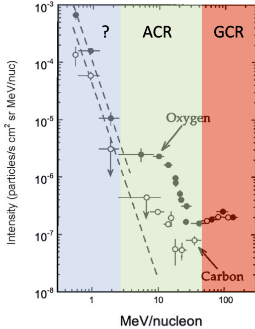
Fig. 1. Quiet-time energy spectra observed near solar minimum at 1.0 au on the Solar, Anomalous, and Magnetospheric Particle Explorer (SAMPEX) satellite in 1992–1993; colored shading approximately separates three energy regimes and their associated spectra. Left: low energy “turn-up” spectra of undetermined origin. Center: anomalous cosmic ray O and C. Right: modulated GCRs. The figure is adapted from Mewaldt et al. (1993).
