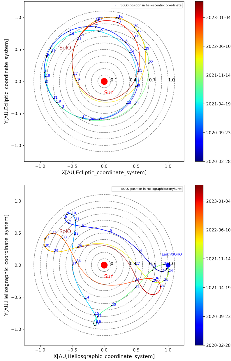
Figure 18: Top: The orbit track of SoLo in the heliocentric mean ecliptic coordinate system where the origin is the center of the Sun, and x-axis points to the mean equinox and the xy - plane is the ecliptic plane. Bottom: The orbit track of SoLo in the Stonyhurst coordinate system. Earth is fixed at 1 au and is marked with a solid blue circle. The other measurements from SOHO/EPHIN, ACE/CRIS/SIS and LND are from locations near Earth. The numbers next to the dashed circle lines indicate the distance from the Sun to 1 au. The blue dots along the track indicate the start of each Carrington rotation of SoLo. About 37 Carrington rotations are used in this study, as the numbers next to the tracks show. The period ranges from February 2020 to May 2023.
