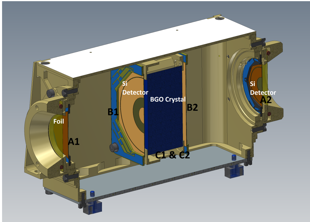
Figure 16: Cut view of HET sensor head. The corresponding detector names are labeled. This figure is reproduced from Rodríguez-Pacheco et al. (2020).
