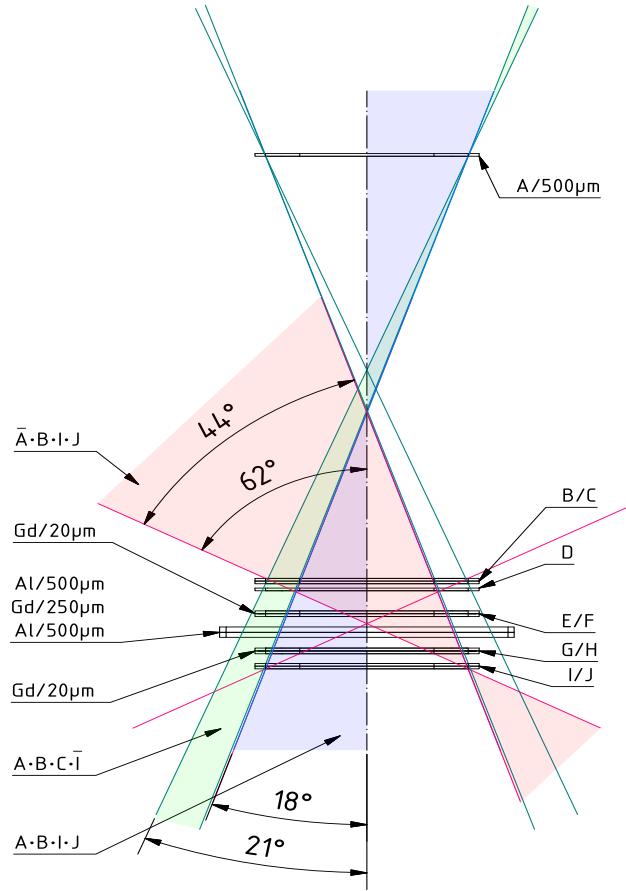
Figure 11: A sketch of the inner structure of the LND SH. Ten 500 \mu\text{m} Si solid state detectors (SSDs) are assembled in order. The different colored regions indicate the field of view (FOV) of different measurement combinations. The figure was reproduced from Wimmer-Schweingruber et al. (2020), and more details could be found in the instrument paper.
