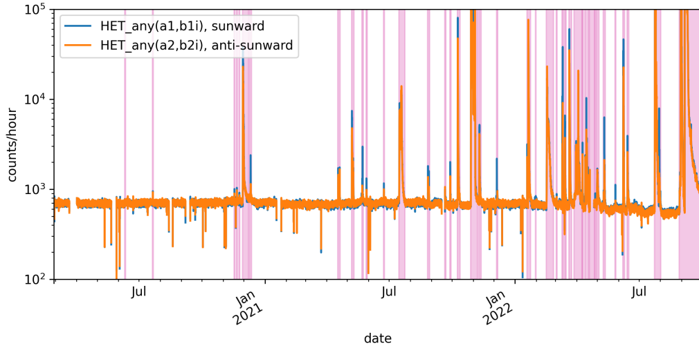
Figure 22: Hourly count rate of the HET multiple detector counters. The magenta-colored regions are the SEP periods we identified.
