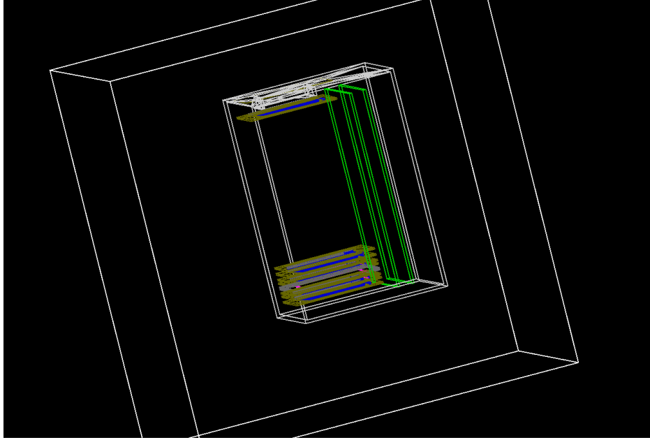
Figure 29: The inner structure of the LND sensor head that is utilized in the Geant4 simulation. The sizes of each piece of structure are taken from the CAD model of LND
