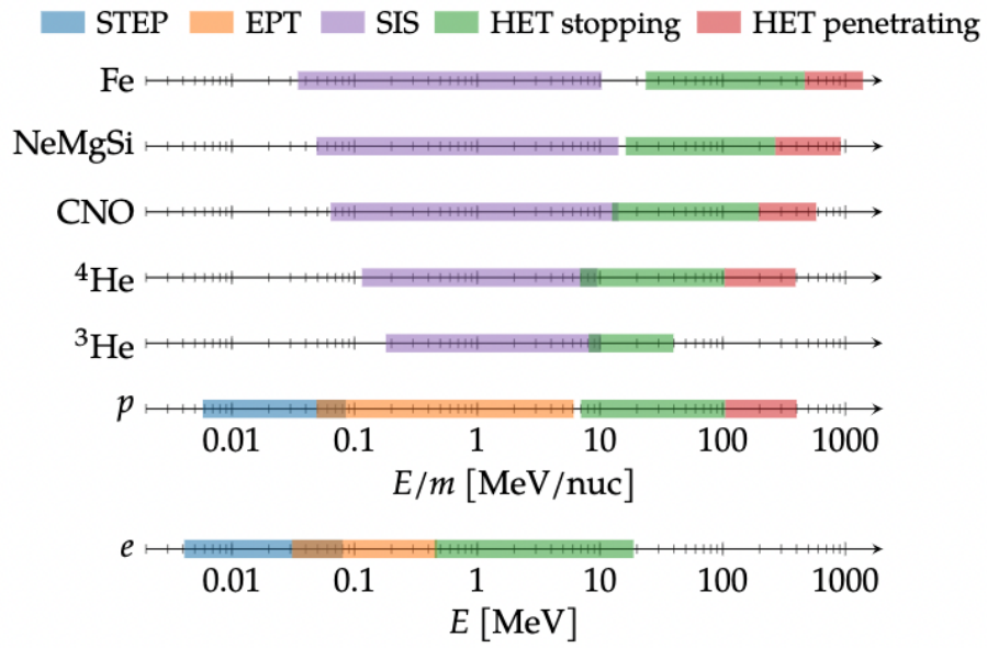
Figure 15: The energy coverage of different EPD sensors for different particle species. This figure is an updated energy coverage plot made by Forstner (2020), based on a similar plot from Rodríguez-Pacheco et al. (2020). The HET measurements are split into stopping and penetrating parts, and the latter one considerably extends HET's capability (Elftmann, 2020).
