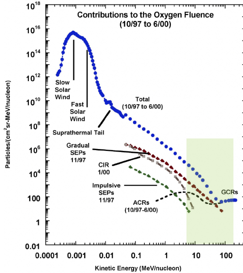
Figure 1: The typical oxygen spectra in the interplanetary space near Earth, indicating the contributions of different particle populations, particularly in the energy range between few MeV/nuc and few hundred MeV/nuc (green shaded region), where SEP, ACR and GCR coexist. The spectra of other particle species, such as, helium and protons, have a similar shape but a different flux level in the corresponding energy regime. The figure is adapted from Mewaldt et al. (2001)
