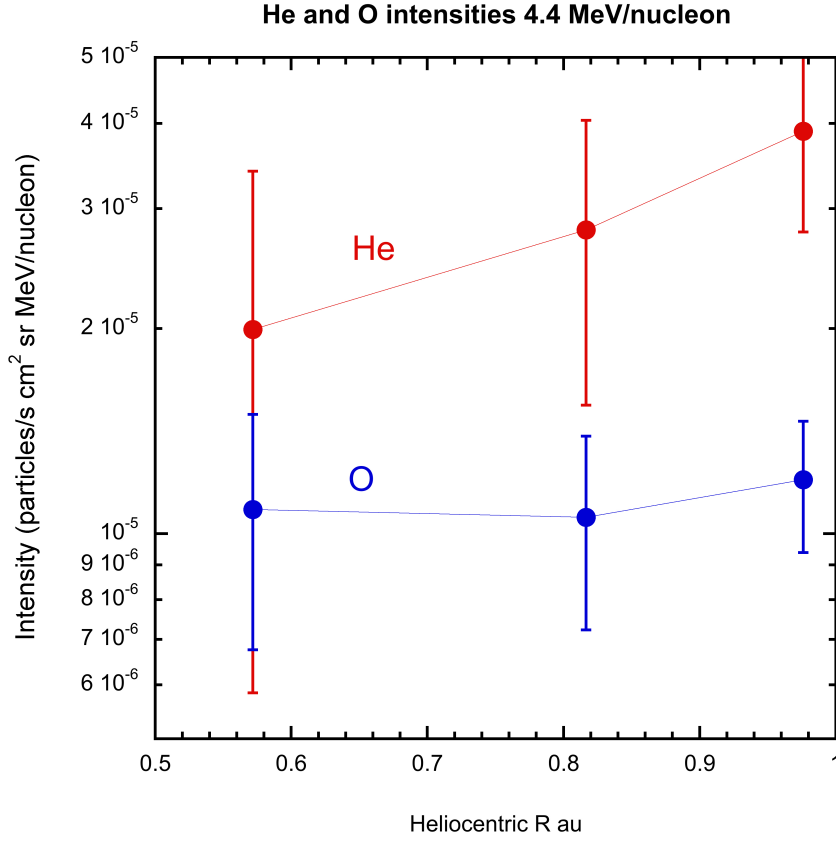
Fig. A.1. Quiet-time interval He and O intensities observed near the peak of the low energy ACR spectra near 4.4\text{ MeV nucleon}^{-1} vs heliocentric radius.
