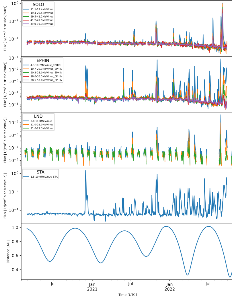
Figure 21: From top to the bottom: The daily averaged helium flux measured by Solo/HET, SOHO/EPHIN, Chang'E-4/LND, and STEREO-A/LET over 2020.2 - 2022.10. The bottom plot shows the radial distance of Solo from the Sun.
