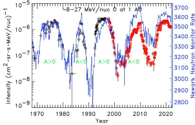
Figure 7: ACR oxygen intensity variation with energy between 8 and 27 MeV/nuc at 1 AU measured by ACE/SIS instrument (red) and count rate of Newark Neutron monitor (blue). The black data points are from the earlier measurements by Mewaldt et al. (1993). (Figure reproduced from Figure 6 of Giacalone et al. (2022))
