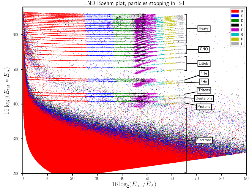
Figure 12: The different particle species are well discriminated in this LND Boehm plot, which is a scatter plot of the LND simulation data generated by the Geant4 tools (Agostinelli et al., 2003). During the simulation, an isotropic source is positioned above detector A.
