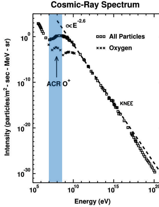
Figure 4: The cosmic-ray spectrum of all particles and anomalous cosmic ray (ACR) oxygen observed at 1 au. This figure is reproduced from Giacalone et al. (2022, 2012), which is originally from Jokipii (1990). The spectrum shows more than 15 orders of magnitude on the energy scale and about 30 orders of magnitude on the intensity scale. In particular, it extends the high energy end of Fig.1. The blue shaded region indicates the energy range that we are interested in this thesis.
