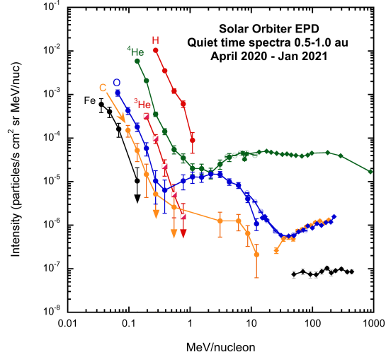
Fig. 2. Quiet-time spectra observed on Solar Orbiter between 0.5 and 1.0 au by EPD/SIS (filled circles and half-filled squares), EPD/HET (filled diamonds), and ACE at 1 au (open circles). Downward pointing arrows signify one-count upper limits.
