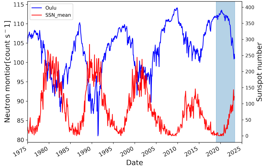
Figure 5: Oulu neutron monitor count rate downloaded from the Neutron Monitor Database (NMDB) measured by the Sodankyla Geophysical Observatory of the University of Oulu, Finland and the monthly averaged sunspot number from Solar Influences Data analysis Center (SIDC), Royal Observatory of Belgium, Brussels. The blue shaded region marks the period that we are interested in.
