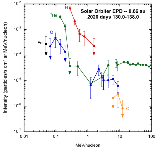
Fig. 3. Low energy spectra during the super-quiet period; symbols are the same as in Fig. 2.
