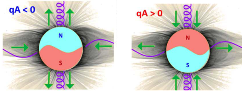
Figure 6: The illustrations of the cosmic ray drift pattern in negative polarity (left) and positive polarity (right). The Sun's north pole has a positive magnetic field, while the south pole has a negative magnetic field during the A > 0 cycle. The signs of the magnetic field in the south and north poles are reversed during the A < 0 cycle. The green arrows indicate the drift directions of ions, and the wavy lines in purple are the heliosphere current sheets. This figure is adapted from the Fig. 4 of Rankin et al. (2022)
