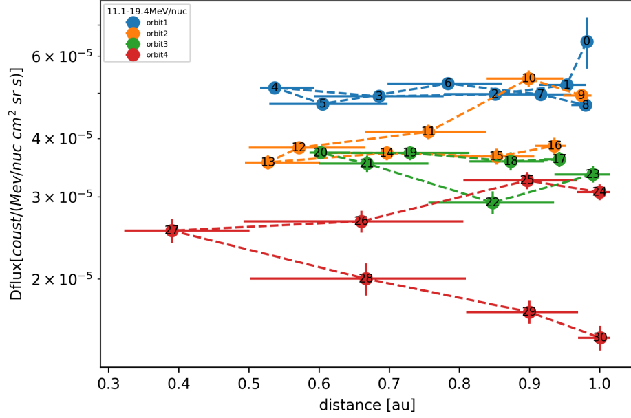
Figure 25: The change of flux of 11.1 - 19.4 MeV/nuc helium from HET with respect to the radial distance of SolO. The data for different orbits are presented in distinct colors. The numbers over data points indicate the order of time.
