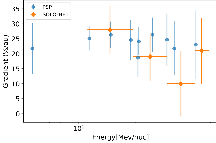
Figure 27: The radial gradient of helium measured in the ecliptic plane at different energies. The values from HET are given as orange diamonds with corresponding error bars. The multiple blue circles in the figure represent the gradient obtained from PSP (Rankin et al., 2021).
