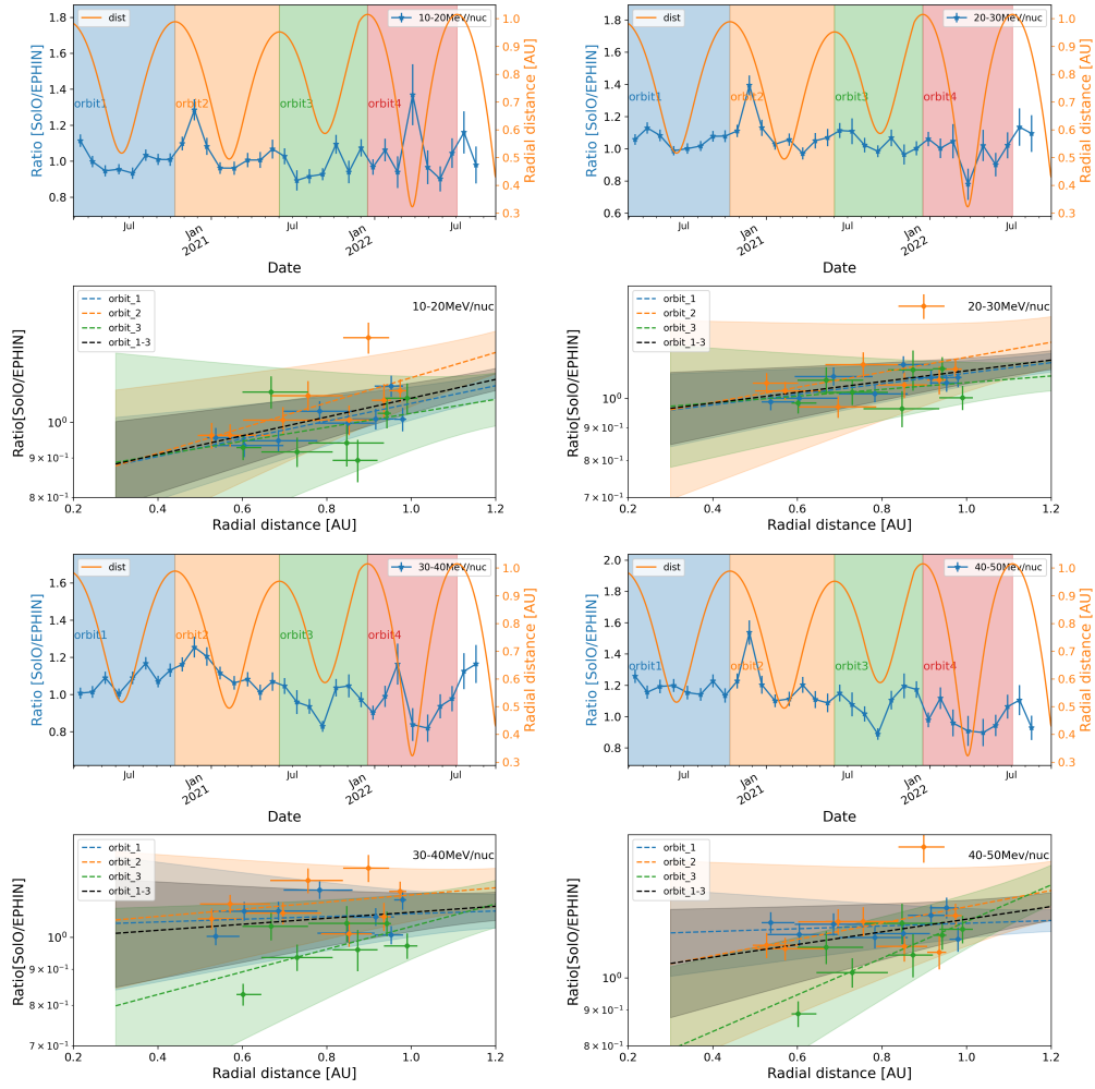
Figure 26: Row 1 and 3: The temporal variation of the helium flux ratio between HET and EPHIN measurements (averaged over their own Carrington rotation and interpolated to calculate the ratio) for different energies; Row 2 and 4: Flux ratio vs radial gradients in the first three orbits, overlay by the log-linear fitting lines.
