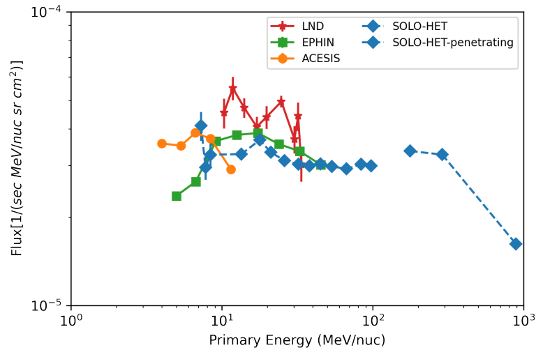
Figure 20: The helium-4 spectra of SolO/HET, SOHO/EPHIN, ACE/SIS and Chang'4/LND when SOLO was between 0.95 and 1AU. SEP events have been removed according to the SEP list in Appendix B.
