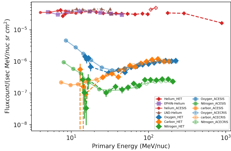
Figure 19: The helium-4 (red, brown, purple), carbon (orange), nitrogen (green), and oxygen (blue) spectra averaged between 2020 and 2022. SEP events have been removed. The data used in this figure covers observations from SolO/HET, SOHO/EPHIN, ACE, and LND.
