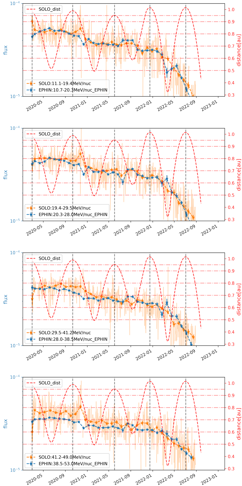
Figure 24: The flux of SolO (orange) and EPHIN (blue) averaged over the Carrington rotation periods in the energy channels of 10 - 20 MeV/nuc, 20 - 30 MeV/nuc, 30 - 40 MeV/nuc, and 40 - 50 MeV/nuc. The daily averaged HET helium fluxes are also shown in different energy channels as light orange lines. Red dashed lines are the radial distance of SolO to the Sun.
