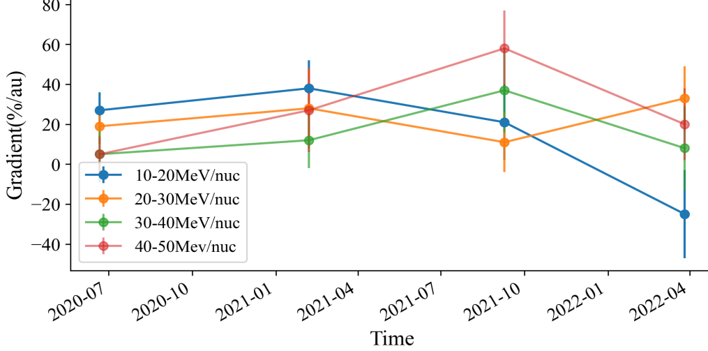
Figure 28: The time variation of the ACR helium radial gradients from 2020 to 2022.
