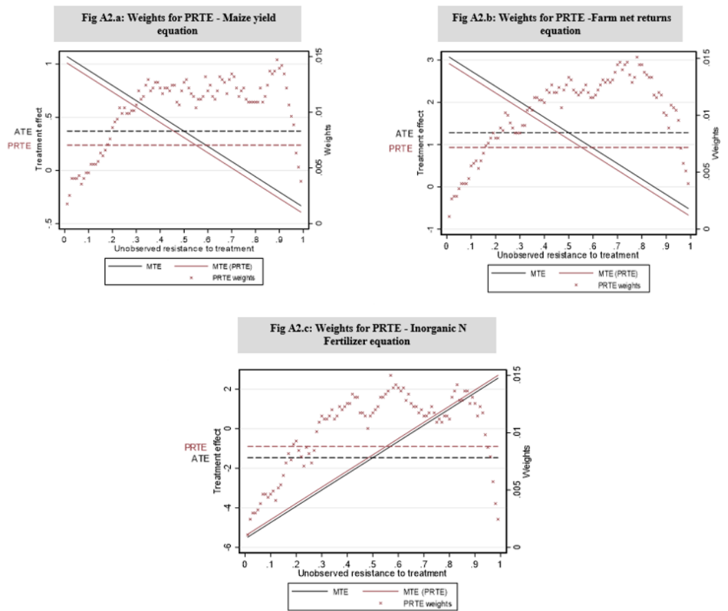
Figure S2. This figure graphs the distribution of the PRTE weights (decreasing CA implementation cost).
