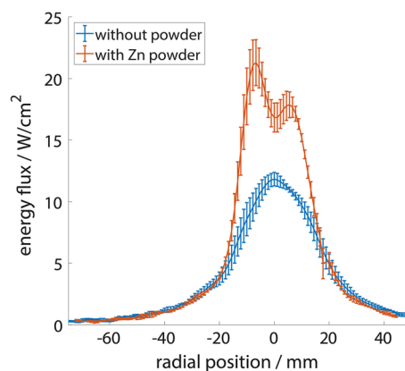
Fig. 10 Comparison of the radial energy flux distribution with and without the addition of Zn powder as precursor for spray coating. (InoCoat, flow 10 slm Ar, current < 100 \text{ A} , axial distance 50 mm, powder rate 6 g/min)
