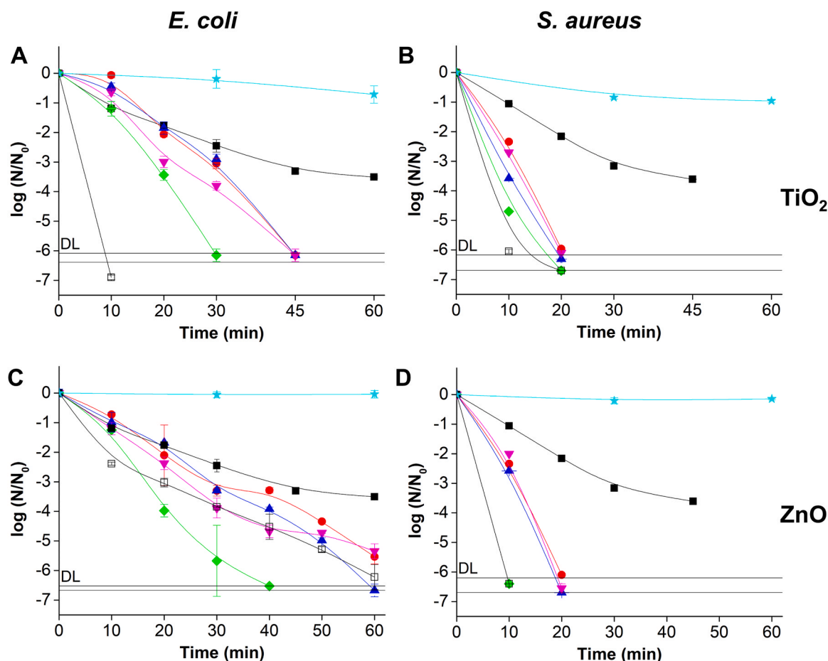
Fig. 4. Solar inactivation of E. coli (A, C) and S. aureus (B, D) with \text{TiO}_2 (A, B) and \text{ZnO} (C, D) photocatalysts as a function of composite loading and semiconductor percentage: dark test with 20 g·L -1 of 80% pellets (—★—), solar inactivation (—■—), and photocatalysis with 0.5 g·L -1 of powdered semiconductor in suspension (—□—) or with 20 g·L -1 of 60% (—●—), 20 g·L -1 of 80% (—▲—), 40 g·L -1 of 60% (—▼—), and 40 g·L -1 of 80% (—◆—) pellets. Natural pH, distilled water, T ca. 30 °C. Note: (—□—) and (—◆—) profiles are fully coincident in Fig. 4D.
