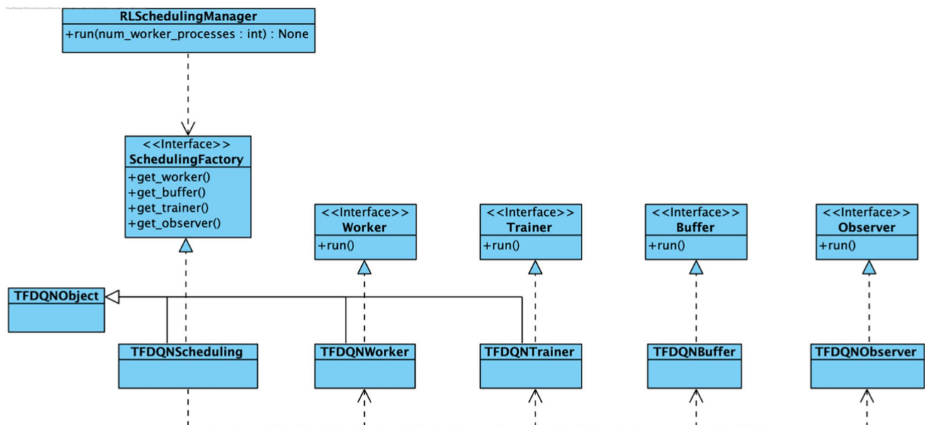
Fig. 12 Creation of the different Processes with the abstract factory design pattern
