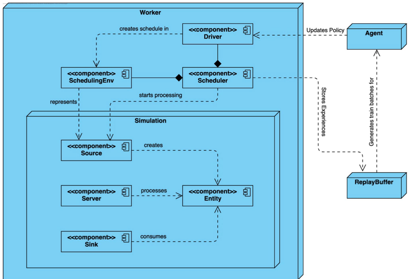
Fig. 11 Deployment diagram illustrating the integration within DMPG
