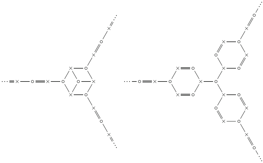
Fig. 2 Two line complexes
