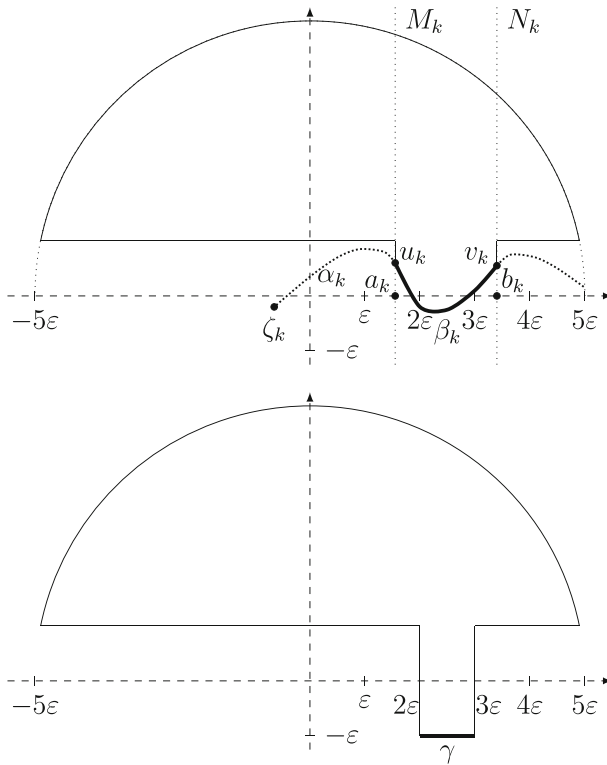
Fig. 1 The curves \alpha_k and \beta_k and the domains G_k (top) and H (bottom)
