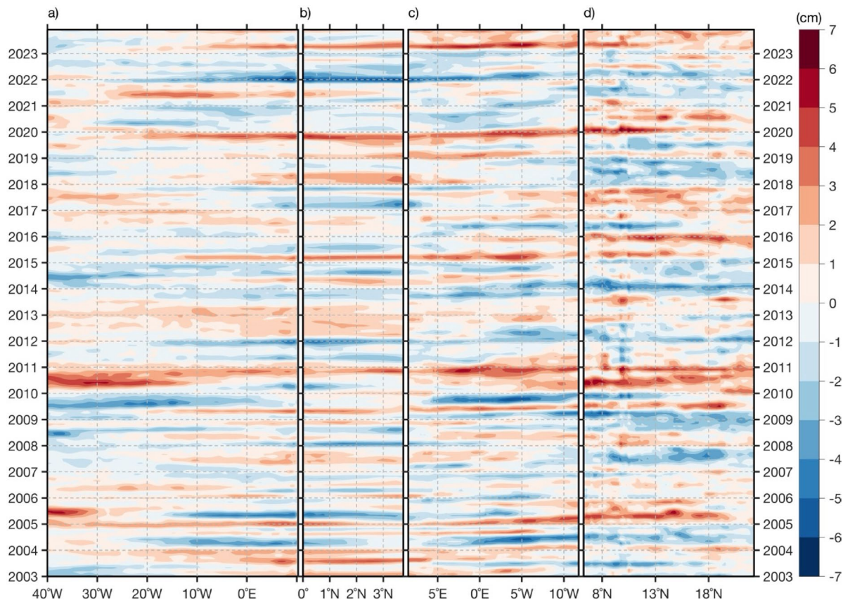
Fig. 7. (a) Hovmoeller diagram of monthly detrended anomalies of SLA along the equator averaged over 1^{\circ}\text{S} - 1^{\circ}\text{N} . (b) Same as (a) with SLA averaged within 1^{\circ} -coastal band from equator to around Cameroon ( 4^{\circ}\text{N} ). (c) Same as (a) but for SLA along the northern coast of the Gulf of Guinea averaged within 1^{\circ} -coastal band along the African coast. (d) Same as (a) but for SLA averaged within 1^{\circ} -coastal band along the northwest African coast from 7.8^{\circ}\text{N} to 24^{\circ}\text{N} . The anomalies are calculated relative to the monthly climatology defined over the period January 2003 to December 2023 with the decadal contribution filtered out using a high-pass Fast Fourier Transform filter with a cut off frequency of 10\text{ year}^{-1} and the subseasonal fluctuations removed by applying a 1-2-1 running weighted average as in Illig et al. 7 .
